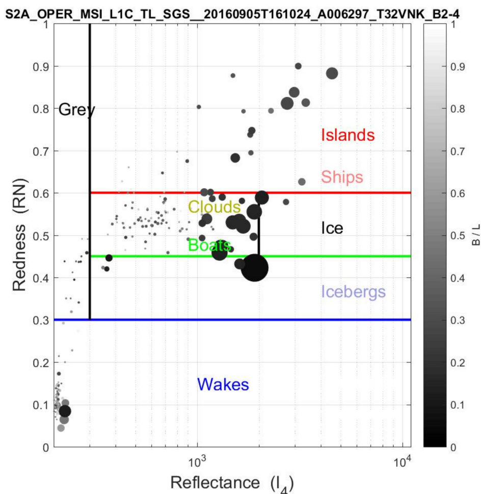
Figure 5. A spectral scatter plot of all segments (mainly ships and wakes) found in Figure 1 distributed according to redness RN vs. average reflectance I_4 . The size of each circle is proportional to the object area A , and its elongation B/L is given by its shading according to the grey level bar on the right. The spectral classifications based on RN and I_4 are shown with text as wakes, grey, ice, and icebergs. The boat vs. cloud and ship vs. island discrimination are based on the spatial separation shown in Figure 4.
