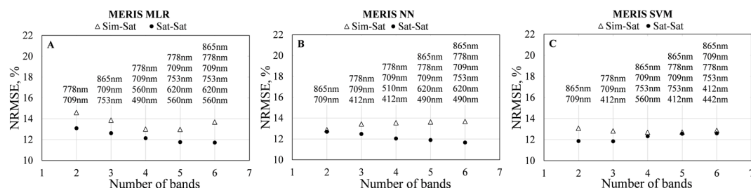
Figure 7. NRMSE of green LAI estimation with different numbers of spectral bands used in MERIS data by (A) multiple linear regression (MLR); (B) neural network (NN); and (C) support vector machine (SVM) regression. Wavelengths corresponding to the centers of the bands used are shown. Each model was trained and validated by different data: Sim-Sat model was trained by data taken at close range, resampled to simulate spectral bands of MERIS and validated by MERIS surface reflectance products; Sat-Sat—trained and validated by MERIS surface reflectance products.
