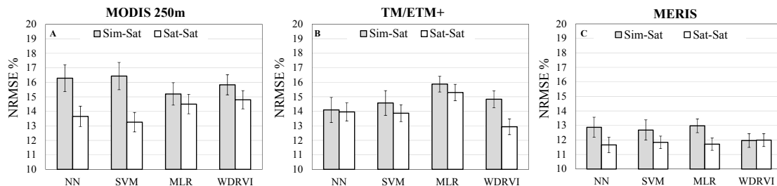
Figure 2. Normalized root mean square errors of green LAI estimation in maize and soybean taken together and their standard deviations (bars) using four techniques (NN, SVM, MLR, and WDRVI) for three satellite sensors: (A) MODIS 250 m resolution; (B) TM/ETM+; and (C) MERIS. Sim-Sat models were trained by reflectance taken at close range resampled to simulate reflectance in spectral bands of satellite sensors and validated by satellite surface reflectance products; Sat-Sat—models were trained and validated by satellite surface reflectance products.
