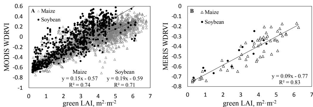
Figure 4. Relationships between (A) MODIS WDRVI and (B) MERIS WDRVI and green LAI in maize and soybean. WDRVI was calculated using MODIS (red and NIR) and MERIS (red edge and NIR) surface reflectance products. The number of points are summarized in Table 1.
