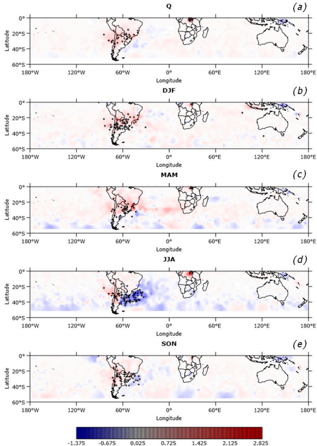
Figure 2. Linear trends (background colours) for the \text{SO}_2 seasonal concentrations in the planetary boundary layer (PBL) (in \text{DU decade}^{-1} ) for (a) Q, (b) December, January, February (DJF), (c) March, April, May (MAM), (d) June, July, August (JJA), and (e) September, October, November (SON). Significant trends are cross-hatched. The level of significance is 95%. Pixels that had at least a seasonal missing value were not included in the analysis.
