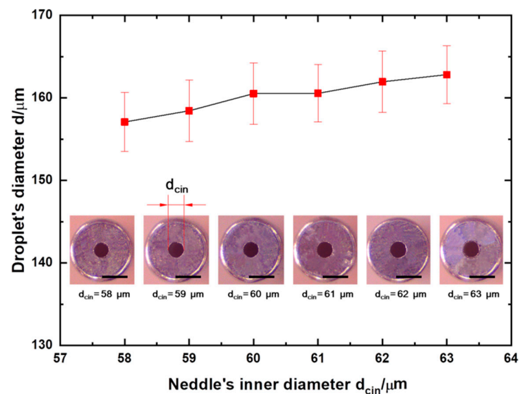
Figure 4. Experiments with different capillary inner diameters. Experiments were carried out when centrifugal acceleration a_{tip} was held constant (108 g). Error bars given are standard deviations (SDs). Scale bars: 100 \mu\text{m} .
