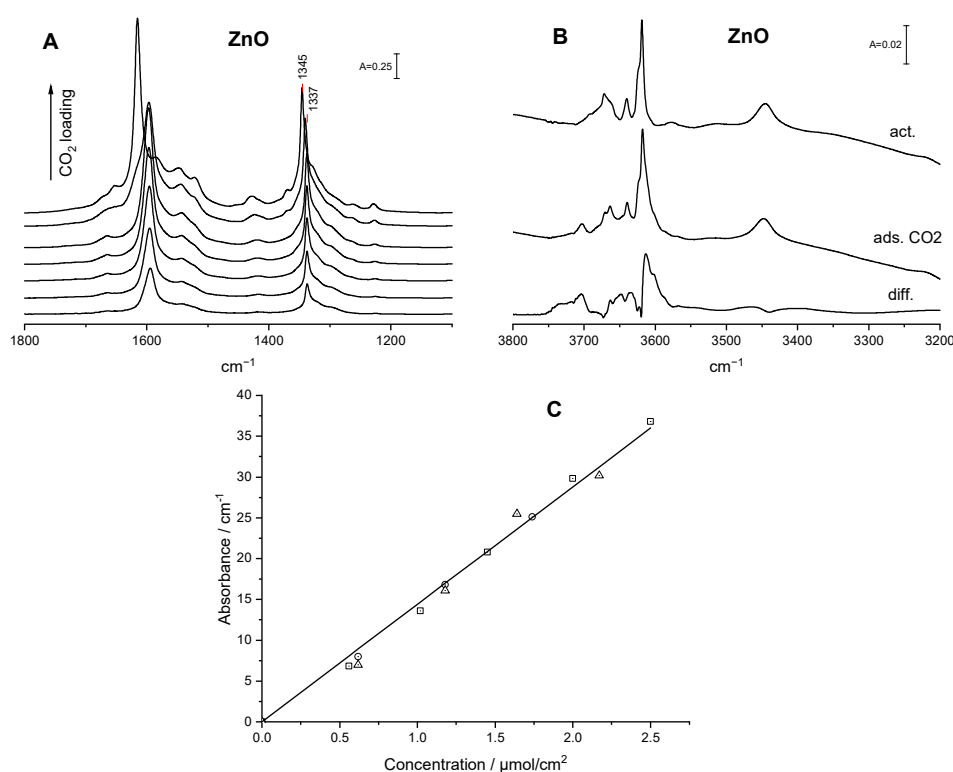
Figure 1. (A)—the spectra recorded upon the adsorption of doses of \text{CO}_2 (ca. 10\text{ }\mu\text{mol/g} ) on \text{ZnO} at RT. (B)—the spectra of OH groups on activated \text{ZnO} , upon \text{CO}_2 adsorption and difference spectrum; (C)—the integrated intensity of the carbonate 1337\text{ cm}^{-1} band as a function of the concentration of adsorbed \text{CO}_2 . \circ\square\triangle represent the results obtained in three independent experiments.
