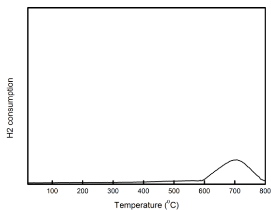
Figure S3. TRP profile for SA-MWCNTs.
