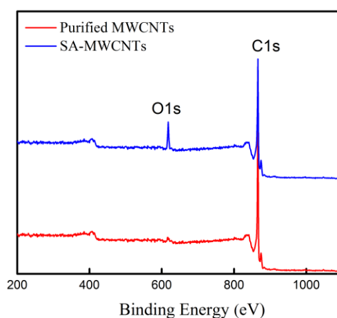
Figure S2. XPS spectra for purified MWCNTs and SA-MWCNTs.
