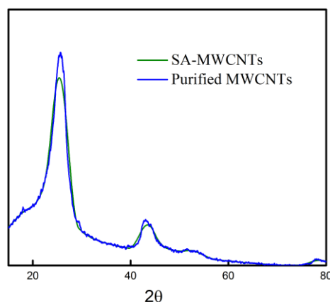
Figure S1. XRD pattern for purified MWCNTs and SA-MWCNTs.
