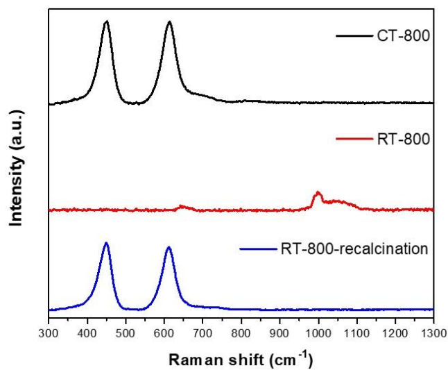
Figure S1. Raman spectra of CT-800, RT-800, and RT-800 recalcination.
