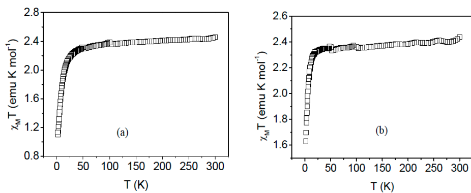
Figure S3. Plots of \chi_m T versus T for 1 (a) and 2 (b).
