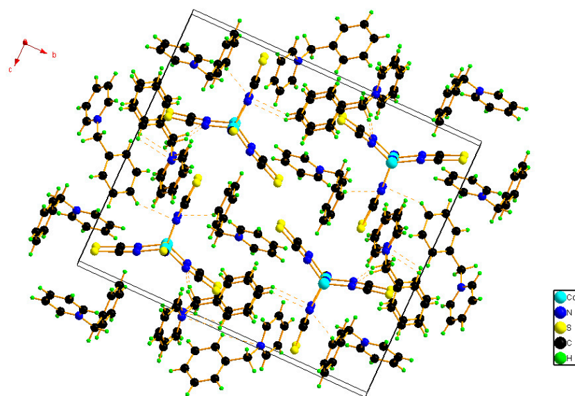
Figure S1. The packing diagram of 1 as viewed along a -axis.
