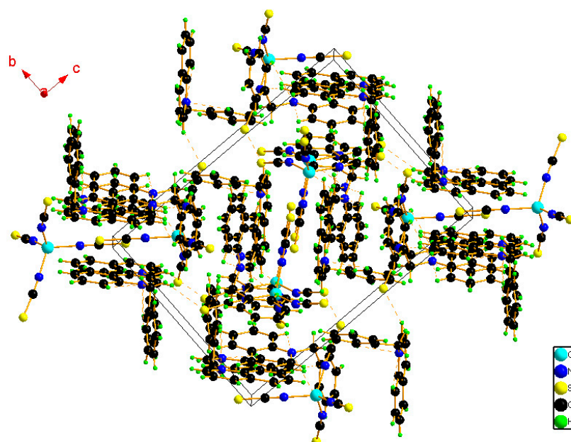
Figure S2. The packing diagram of 2 as viewed along a -axis..
