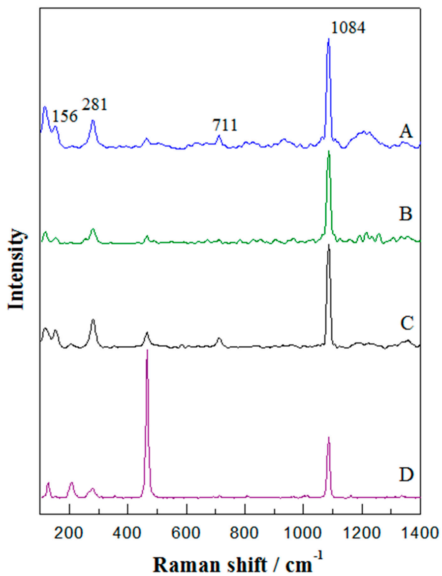
Supplementary 1: The Raman analysis of upper (A) and bottom (B) sections for monoculture, and upper (C) and bottom (D) sections for coculture.
