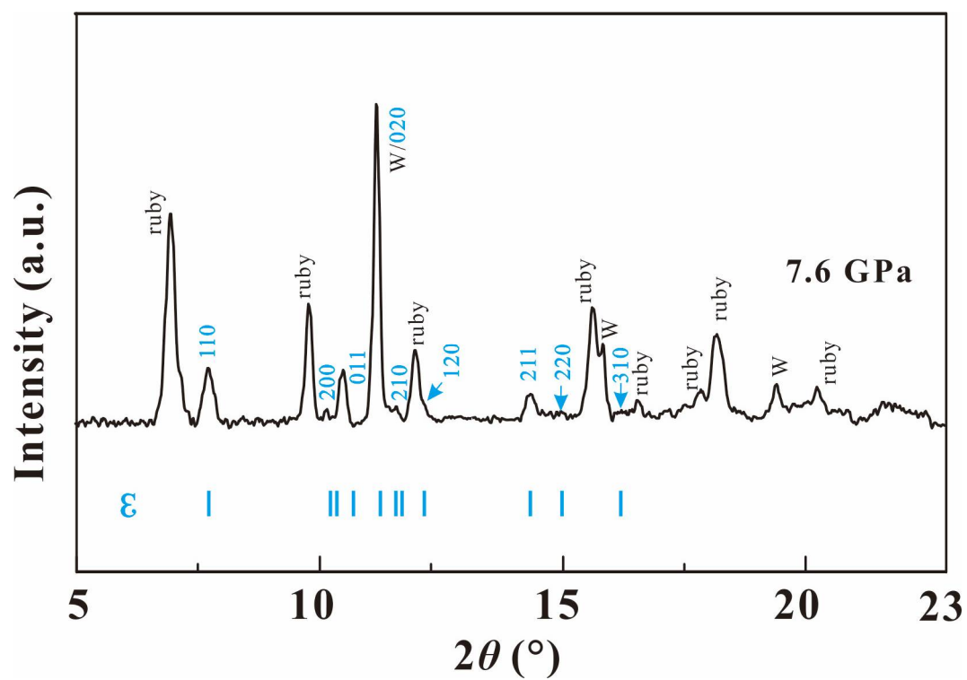
Figure S1. Selected x-ray diffraction patterns of compressed \epsilon -FeOOH under non-hydrostatic condition.
