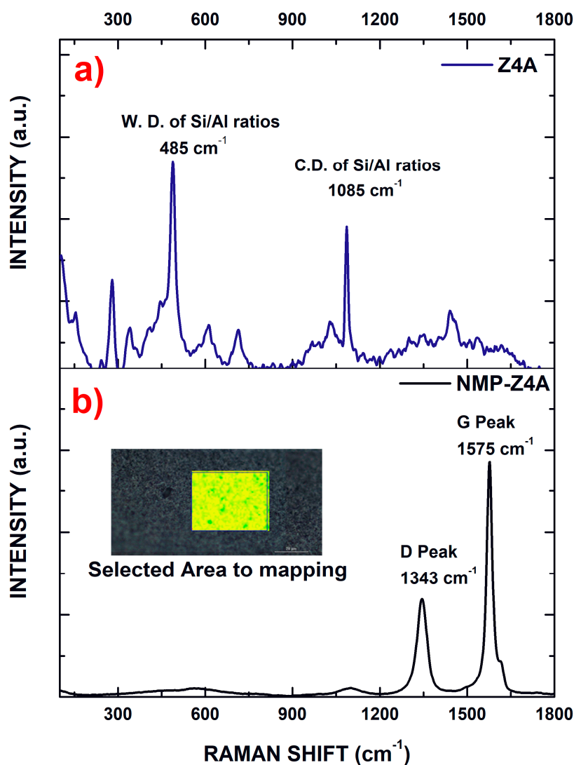
Figure S1. Raman spectrum of (a) zeolite 4A (Z4A) and (b) graphene dispersed in NMP+Z4A after centrifugation for 10 min at 1000 rpm. (Inset) Sampled region.
