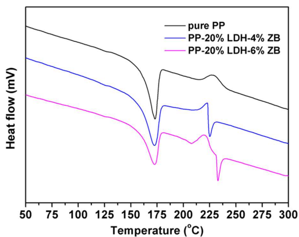
Figure S1. DSC curves (exo up) of the pure PP and PP/LDH/ZB composites.
