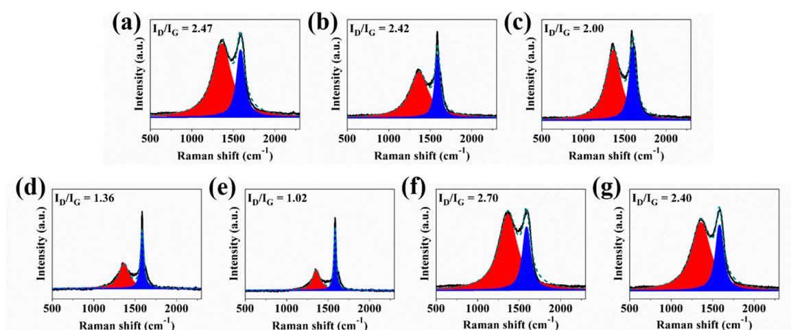
Figure S1. Raman spectra of external char residues of (a) RPUF-1, (b) RPUF-2, (c) RPUF-3, (d) RPUF-4, (e) RPUF-5, (f) RPUF-6, and (g) RPUF-7 after cone calorimeter testing.
