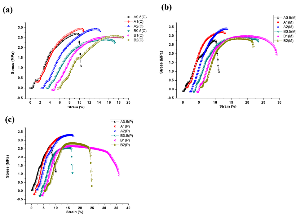
Figure S1. Selective stress-strain curves of different samples molded by (a) CIM, (b) MFVIM, and (c) PVIM.
