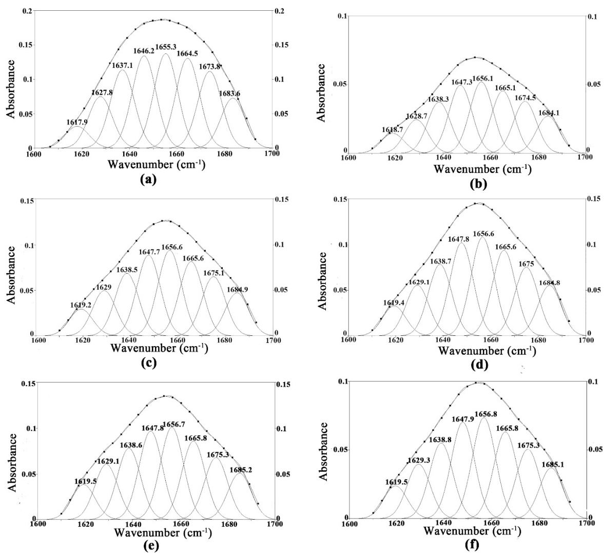
S 2. Second-derivative FTIR spectra in the amide I region and Gaussian curve fitting. (a) Pv; (b) Za; (c) Zb; (d) Zc; (e) Zd; (f) Ze.
