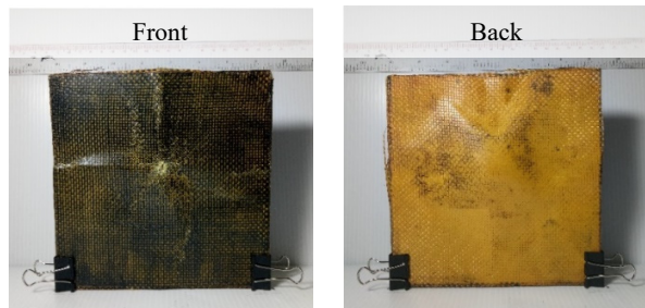
20 plies of aramid fabric reinforced PBA/PU filled with MWCNT
