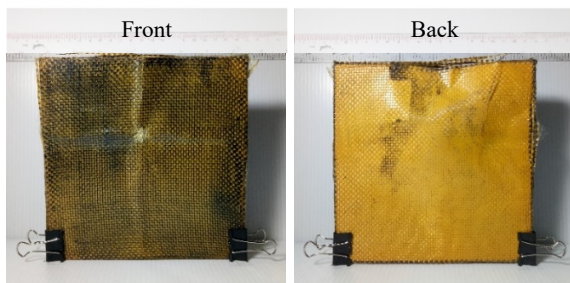
20 plies of aramid fabric reinforced PBA/PU filled with MWCNT
