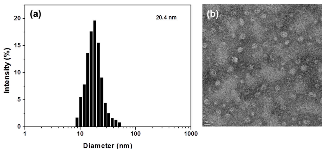
Figure S1. (a) Dynamic light scattering (DLS) diagram of DOX-loaded micelles; and (b) transmission electron microscopy (TEM) image negatively stained with phosphotungstic acid hydrate (scale bar, 20 nm).
