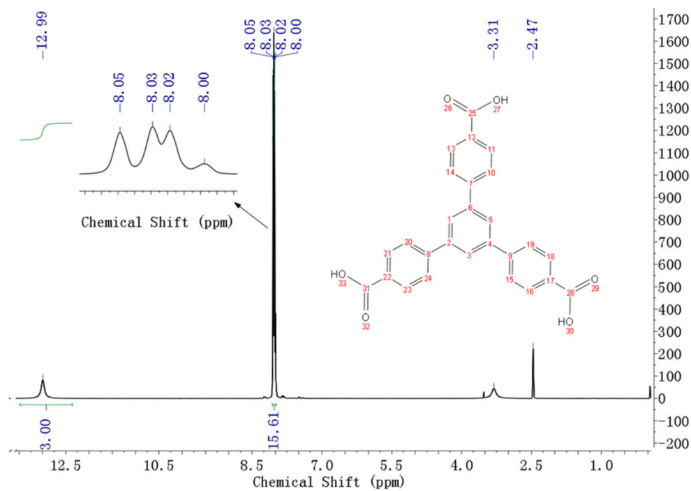
Figure S3. 1 H NMR spectrum of H 3 BTB.
