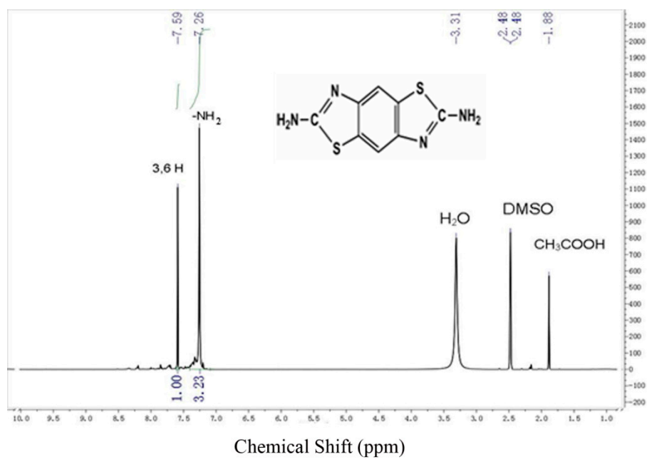
Figure S1. 1 H NMR spectrum of DABBT.
