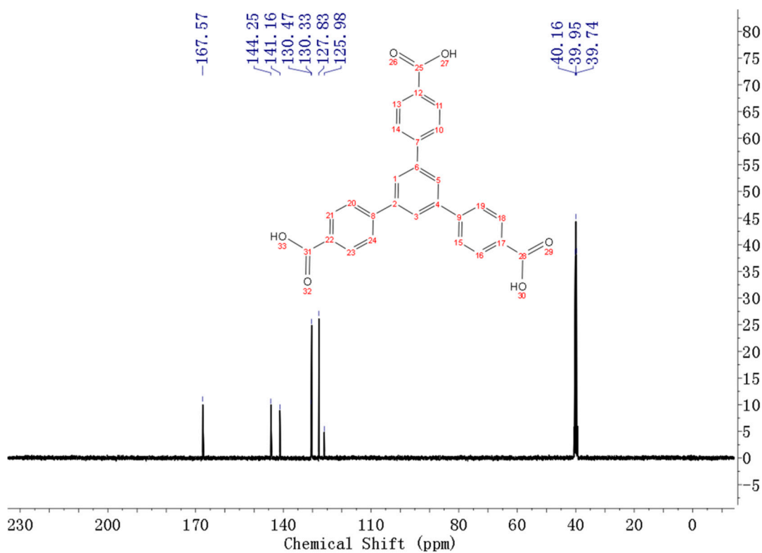
Figure S4. 13 C NMR spectrum of H 3 BTB.
