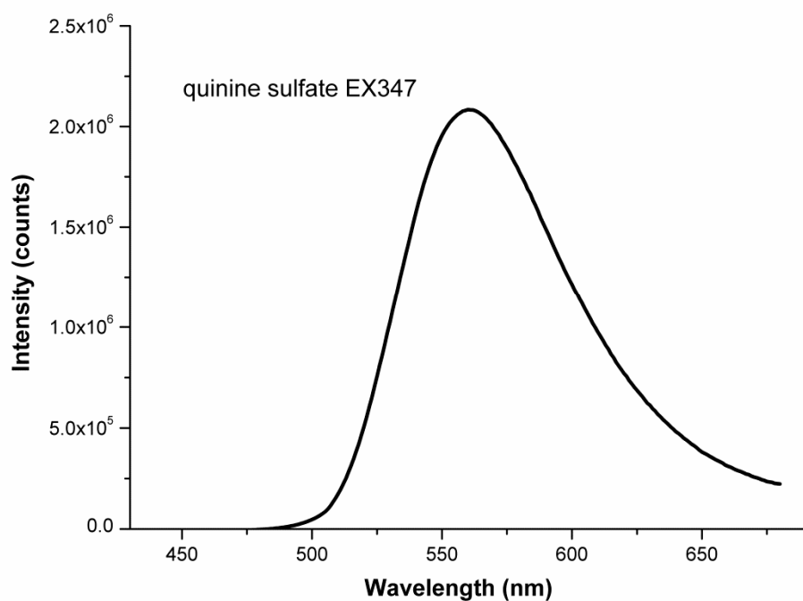
Figure S6. Fluorescent spectrum of quinine sulfate in 0.1M H 2 SO 4 .
