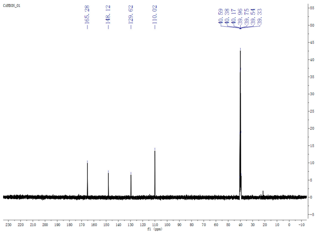
Figure S2. 13 C NMR spectrum of DABBT.
