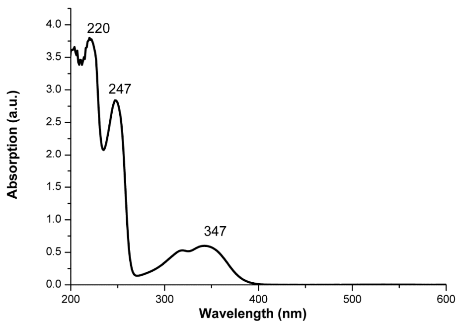
Figure S5. UV-vis absorption spectrum of quinine sulfate in 0.1M H 2 SO 4 .
