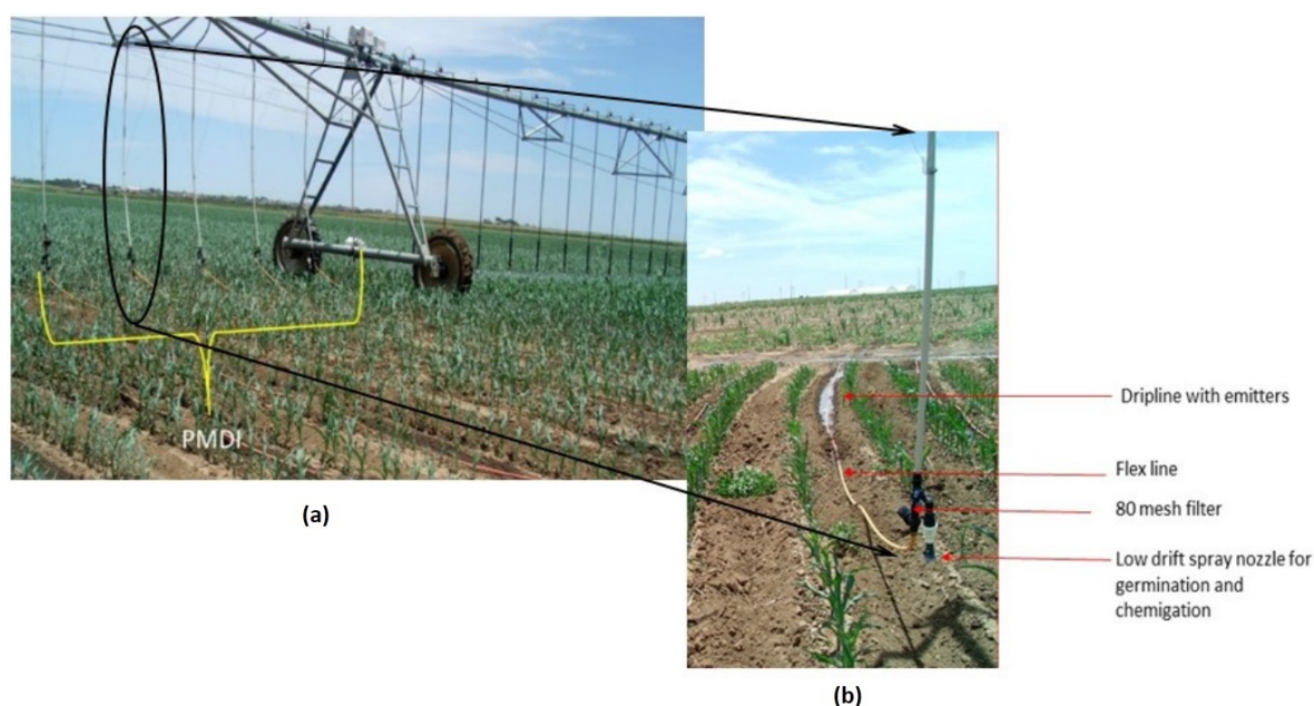
Figure 4. Precision mobile drip irrigation (MDI) system: (a) shown on span 1 to the left; and (b) zoomed-in view of one MDI drop showing sprinkler hardware, filter and dripline dragging between.
