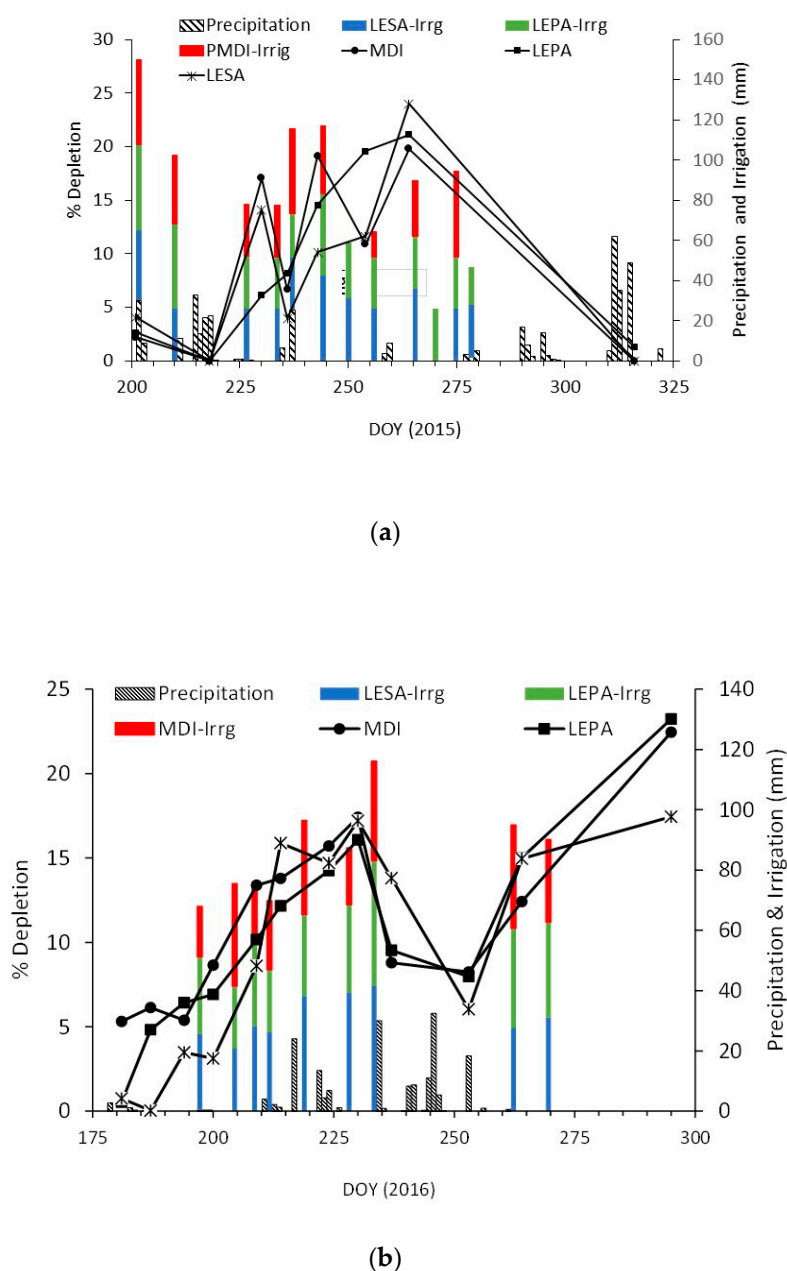
Figure 1. Average percent soil water depletion in the top 1.5 m depth (calculated using Equation (2)) of treatment plots for mobile drip irrigation (MDI), low energy precision application (LEPA) and low elevation spray application (LESA) methods during: (a) the 2015 and (b) 2016 growing seasons.
