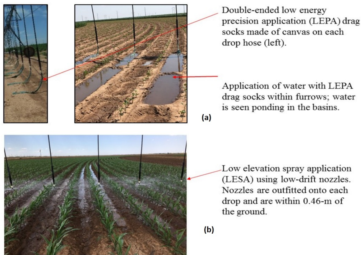
Figure 3. Application methods commonly used on center pivot systems in the Texas High Plains region (a) low energy precision application (LEPA); and (b) low elevation spray application (LESA).
