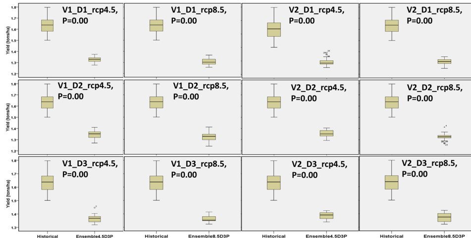
Figure 8. Samaru maize yield ensemble (9 GCMs) for poor fertility under RCP4.5 and 8.5 for future period, 2021/25–2050 relative to the baseline period, 1981/85–2010.
