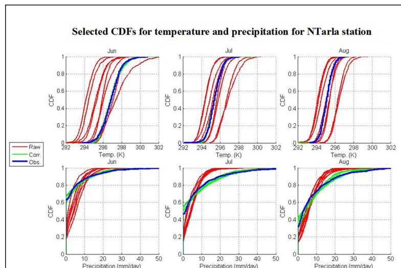
Figure 3. Cumulative distribution functions (CDFs) for the N'Tarla station. Minimum daily temperatures are in the top panel while precipitation values are in the bottom. Red CDFs are raw model data, green CDFs are bias corrected and blue CDFs are observed.
