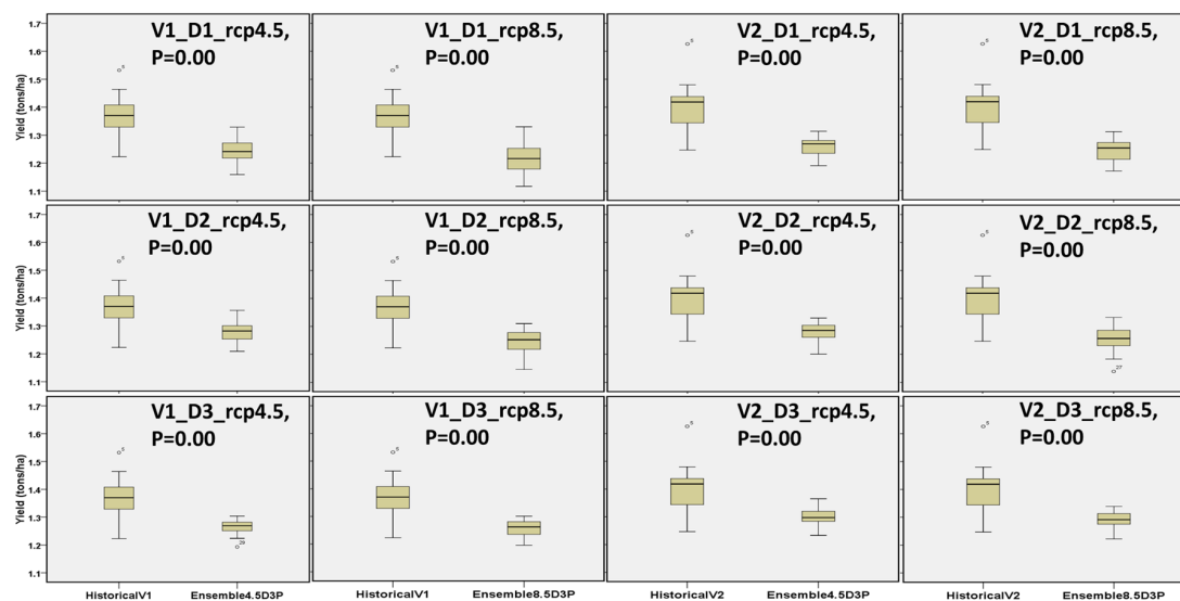
Figure 10. Samaru sorghum yield ensemble (9 GCMs) poor fertility under RCP4.5 and 8.5 for future period, 2021/25–2050 relative to the baseline period, 1981/85–2010.
