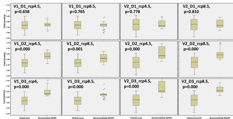
Figure 7. Makurdi sorghum yield ensemble (9 GCMs) for poor fertility under RCP4.5 and 8.5 for future period, 2021/25–2050 relative to the baseline periods, 1981/85–2010.
