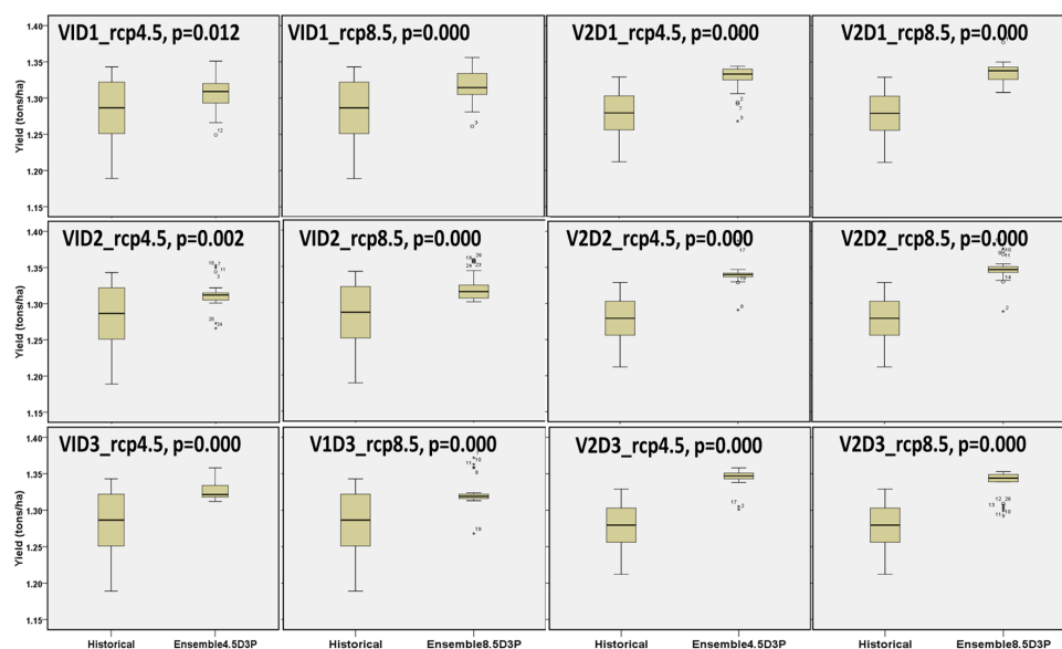
Figure 6. Makurdi maize yield ensemble (9 GCMs) for poor fertility under RCP4.5 and 8.5 for future period, 2021/25–2050 relative to the baseline period, 1981/85–2010.
