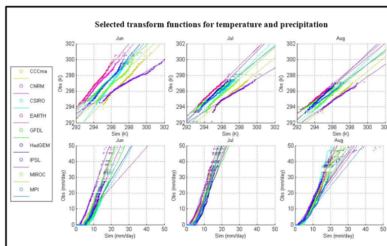
Figure 2. Bias correction transform functions for temperature (top panels) and precipitation (bottom panels).
