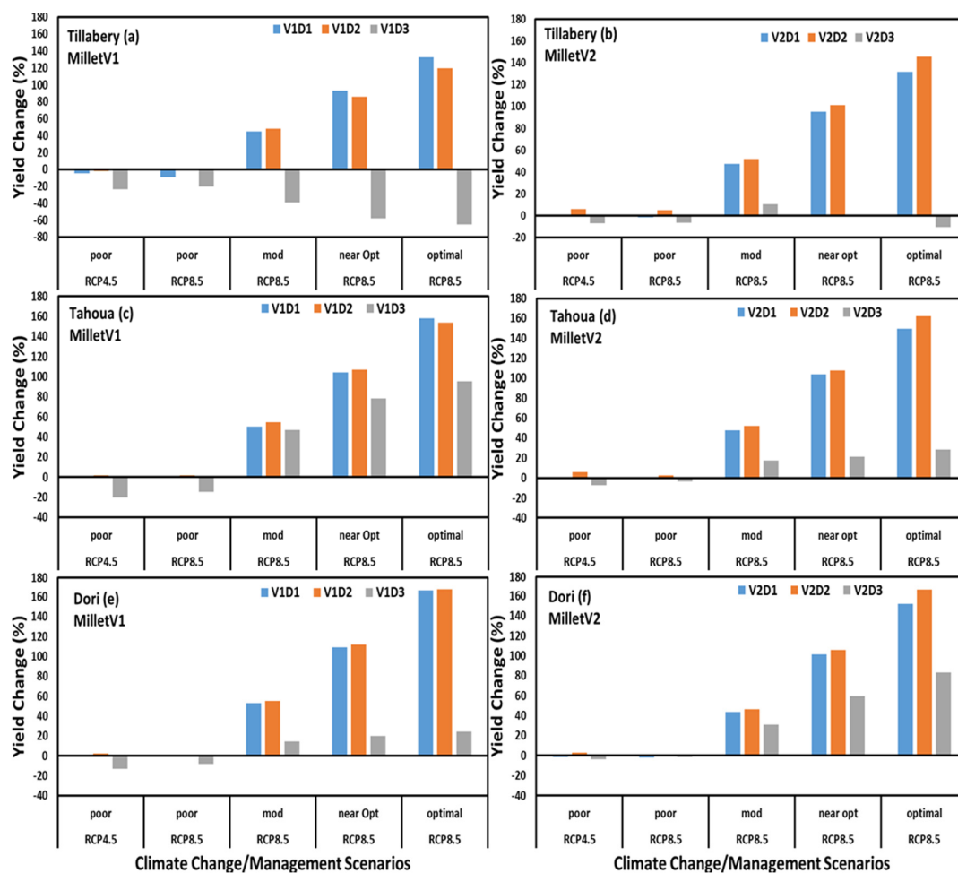
Figure 11. Millet yield ensemble (9 GCMs) change under RCP4.5 and 8.5 scenarios for future period, 2021/25–2050, relative to the baseline period, 1981/85–2010.
