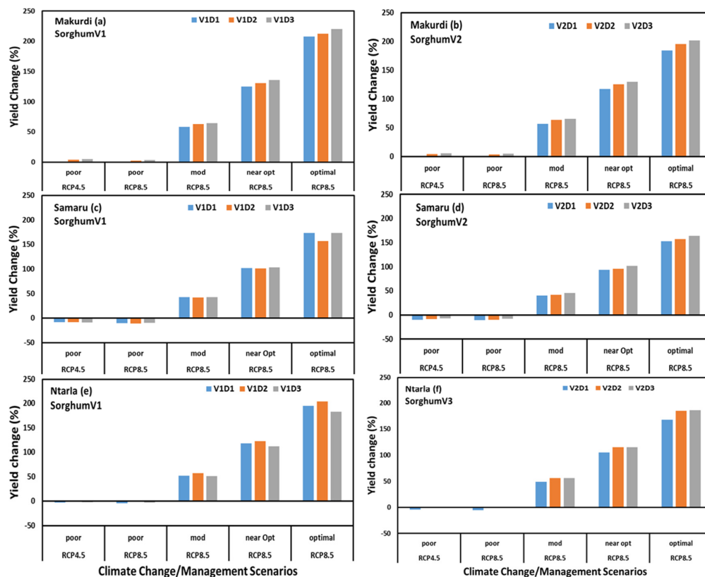
Figure 9. Sorghum yield ensemble (9 GCMs) change under RCP4.5 and 8.5 scenarios for future period, 2021/25–2050 relative to the baseline period, 1981/85–2010.
