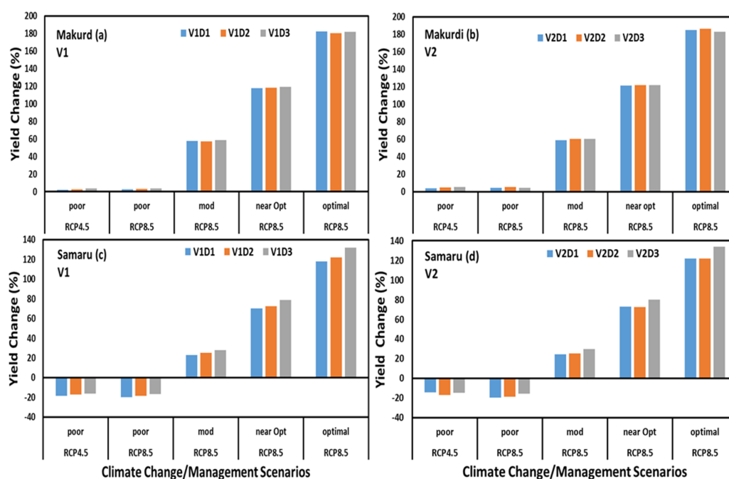
Figure 5. Maize yield ensemble (9 GCMs) change under RCP4.5 and 8.5 scenarios for future period, 2021/25–2050 relative to the baseline period, 1981/85–2010.
