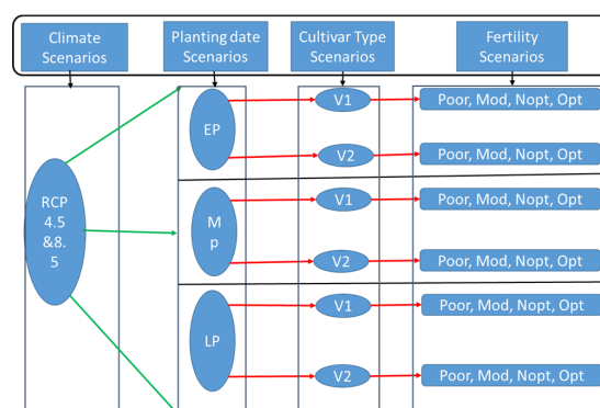
Figure 4. Flowchart showing the various climate change adaptation scenarios. Note, EP = early planting (D1); MP = mid planting (D2); LP = late planting (D3); V1 = long duration (110–125 DAP); V2 = medium duration cultivar (105–110); Mod = moderate fertility; Nopt = near optimal fertility; and Opt = optimal fertility. Note: Sorghum V1 = 130–145 DAP; V2 = 110–125, DAP.
