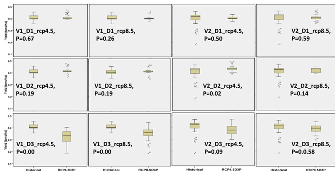
Figure 12. Tahoua millet yield ensemble (9 GCMs) for poor fertility under RCP4.5 and 8.5 for future period, 2021/25–2050 relative to the baseline period, 1981/85–2010.
