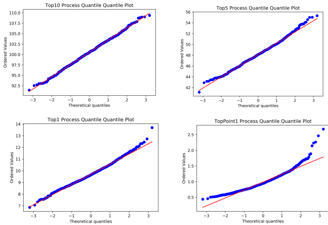
Figure S3. Quantile-Quantile Plots for the PENs. Quantile-quantile plots for each null distribution of the thresholded Predictive Expression Networks. .
