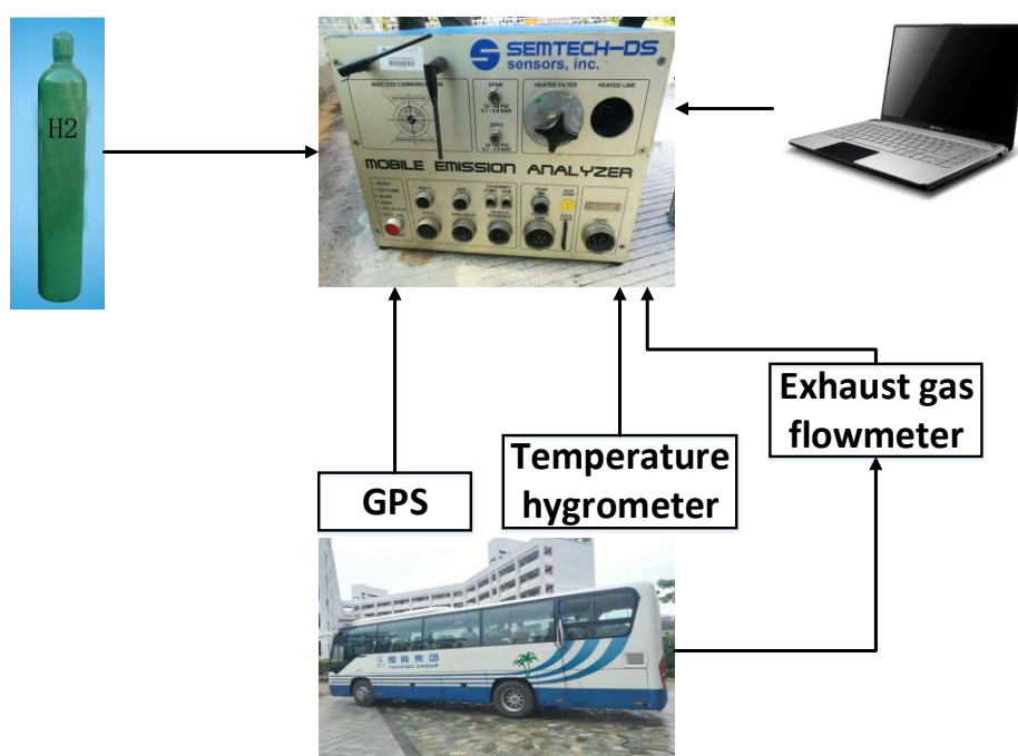
Figure S2. Portable emission measurement system schematic.
