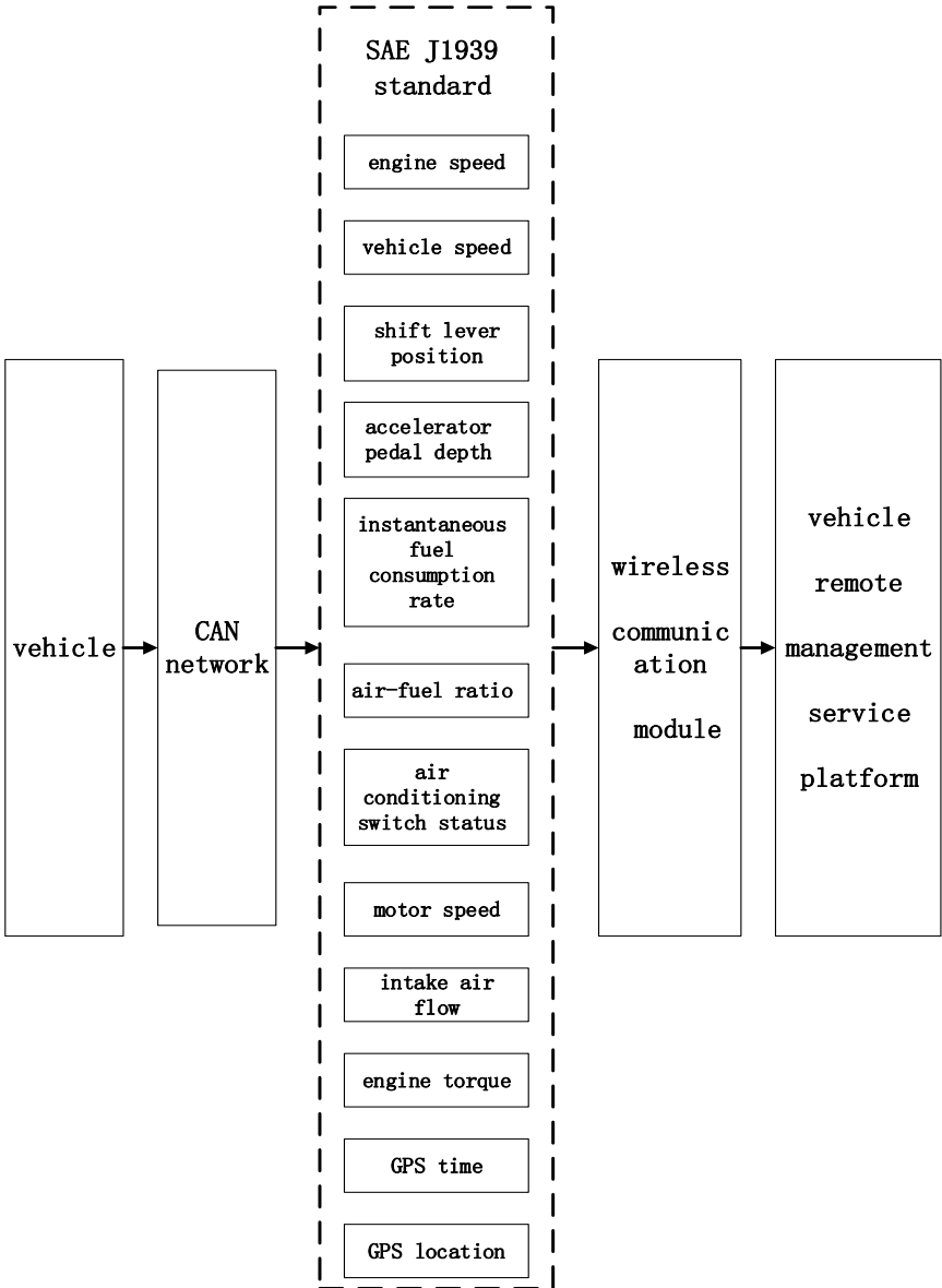
Figure S1. Road test remote information system and data analysis process.
