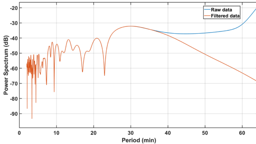
Figure S1. The power spectrum of a pressure for the time series. Blue line represents pressure data and red line represents filtered pressure data
