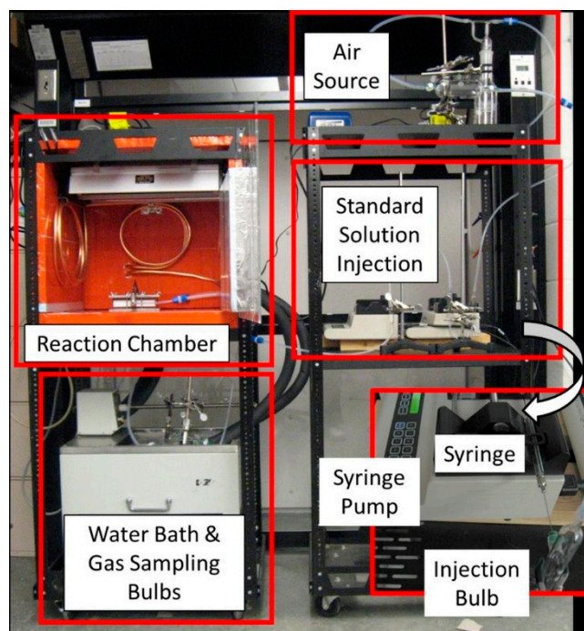
Figure S1. Photo of the laboratory-scale set-up for testing the effects of light and special coatings on standard gas mixtures of volatile organic compounds (in this photo, the system is rolled outside of the walk-in fume hood. All tests were completed inside the hood). The bottom photo is a close-up of the standard gas mixture to air pumped through the system. (Iowa State University Air Quality Lab).
