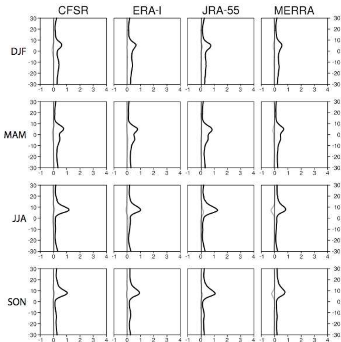
Supplemental Figure S1. The black curves are the zonal averages of precipitation from Figure 7a (western hemisphere tropics; 30° N–30° S and 180°–0° W) for each reanalysis model (labeled at top) and for each season (labeled at left) over the 1981–2010 period. The gray curves show the differences of the ensemble subtracted from the reanalysis model. The thin black lines mark zero difference. The y-axes left and right represent degrees latitude.
