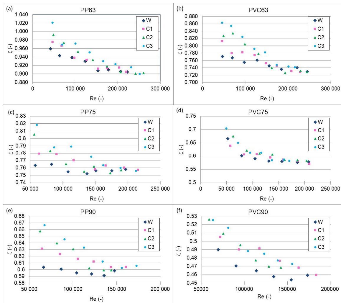
Figure 4. Values of coefficient \zeta as a function of Reynolds number Re and concentration of sand for the test elbows. Elbows: (a,b)—diameter 63 mm, (c,d)—diameter 75 mm, (e,f)—diameter 90 mm.
