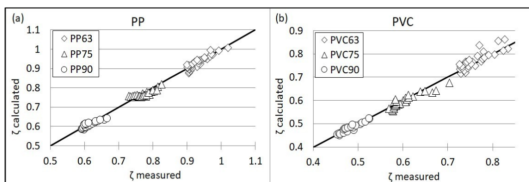
Figure 12. Verification of the correctness of the adopted model for PP (a) and PVC (b) elbows as a function of diameter d , concentration of suspended solids C , and Reynolds number Re .
