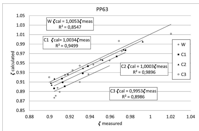
Figure 11. Verification of the correctness of the adopted model for the PP63 elbow.
