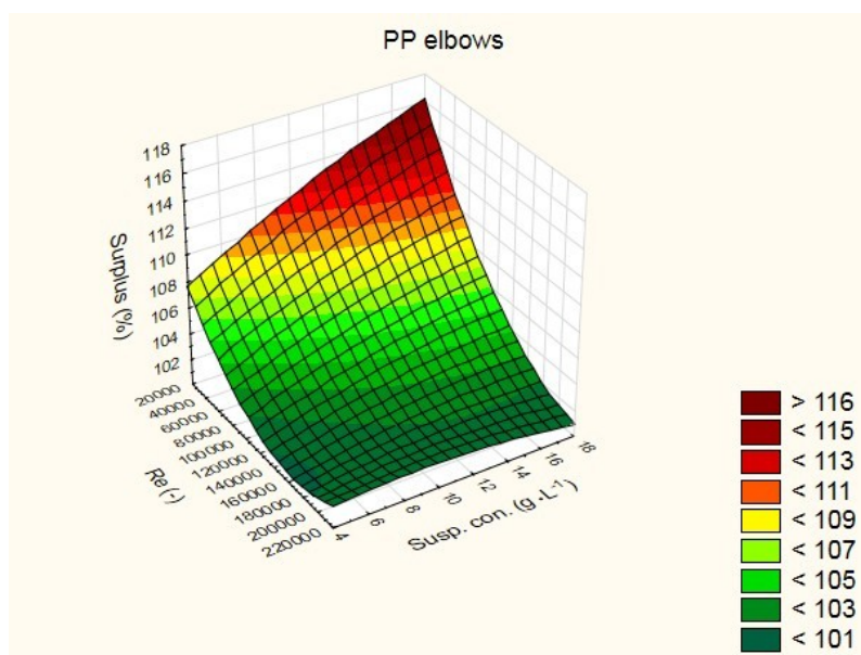
Figure 9. Increase in head loss through PP elbows for water-sand mixtures compared to clear water, as a function of sand concentration and Reynolds number.
