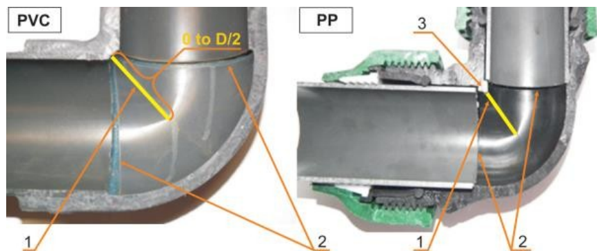
Figure 6. Longitudinal section of the test elbows: 1—inner edge of the elbow, 2—edge of the joint, 3—inner notch.
