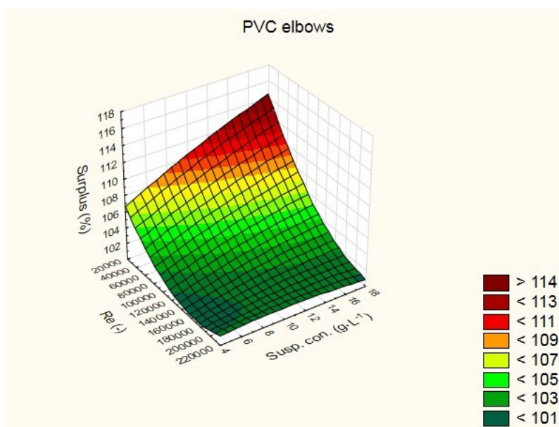
Figure 10. Increase in head loss through PVC elbows for water-sand mixtures compared to clear water, as a function of sand concentration and Reynolds number.
