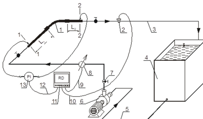
Figure 1. Schematic of the test stand for measuring minor head losses through elbows: 1—elbow, 2—thermometer, 3—pipe supplying sewage to the tank, 4—sewage tank, 5—pipe channeling sewage from the tank, 6—sewage pump, 7—needle valve, 8—sewage flow meter, 9, 10 and 12—control cable, 11—data recorder, 13—differential pressure meter, 1–1; 2–2—test cross-sections, L_1 , L_2 —distance of measuring cross-sections to the elbow.
