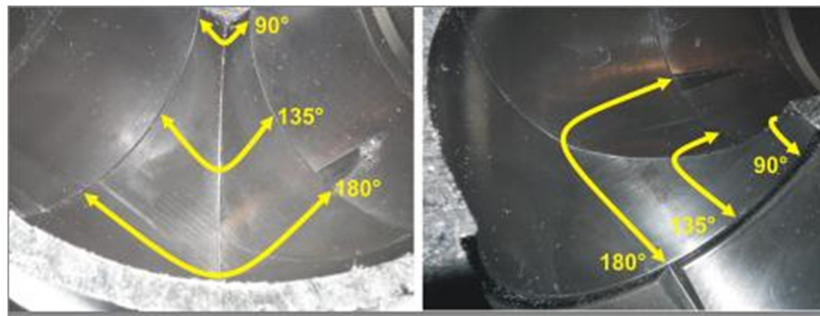
Figure 7. Flow deflection angle on the inner edge of an elbow.
