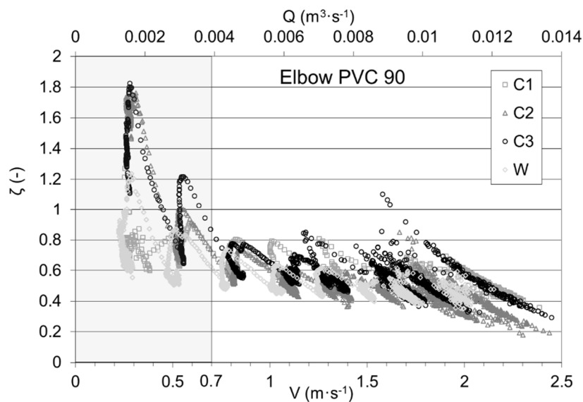
Figure 3. Minor head loss coefficient \zeta for a PVC90 elbow as a function of water flow velocity and three concentrations of water-and-sand mixture.
