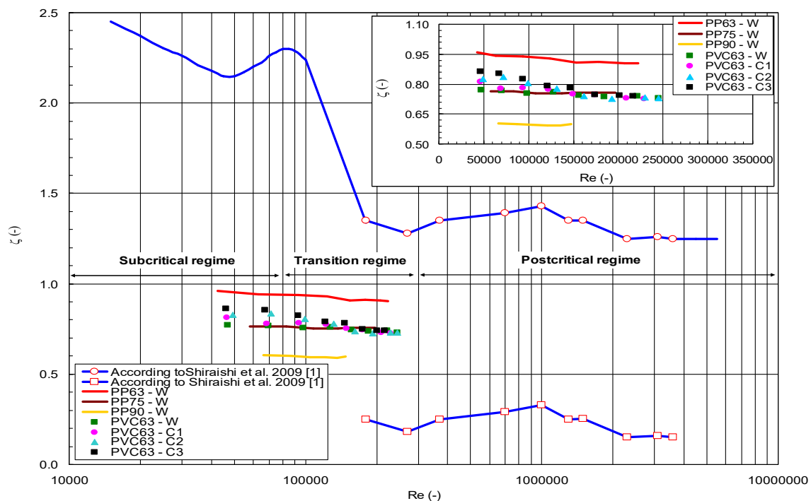
Figure 5. Comparison of experimental data for \zeta with the correlation found by Shiraishi et al. (2009) [1].
