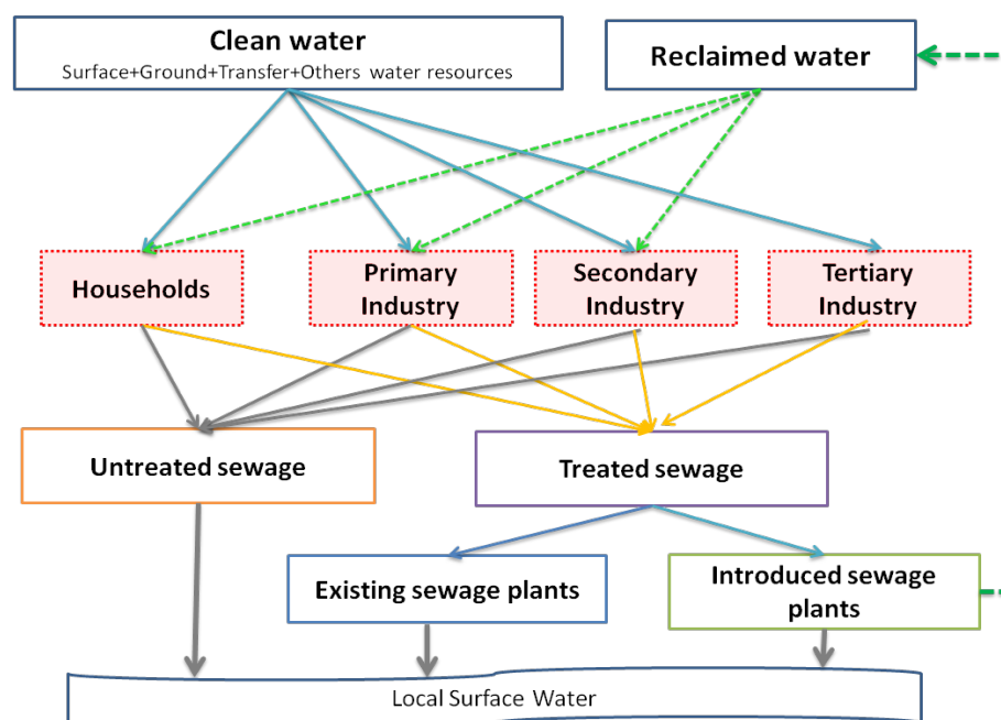
Figure 2. Water flow in water resources cycle system.
