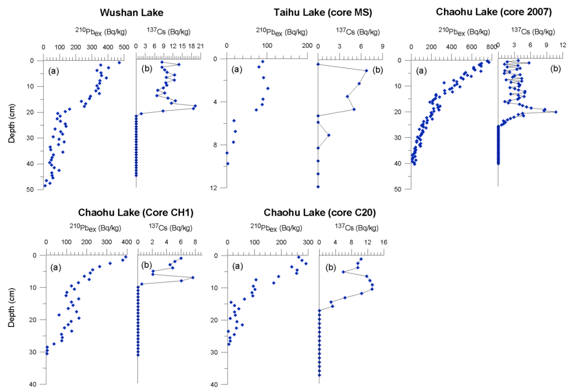
Figure S1. Unsupported ^{210}\text{Pb} (CRS model) activity and ^{137}\text{Cs} activity for 15 cores in 11 lakes.
