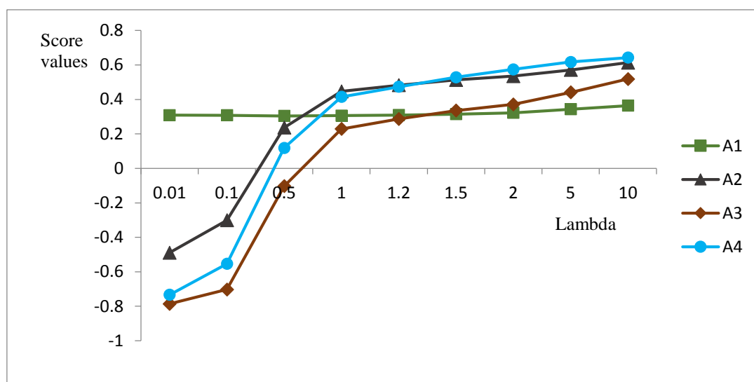
Figure 1. Ranking sensitivity analysis based on different parameter \lambda in NIFGWPIA operator.
