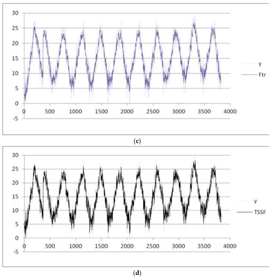
Figure 11. (a) Results obtained for the variation of the mean temperature by using the avgSV method; (b) results obtained for the variation of the mean temperature by using the ARIMA method; (c) results obtained for the variation of the mean temperature by using the F-transforms method; and (d) results obtained for the variation of the mean temperature by using the TSSF method.
