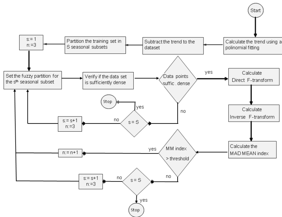
Figure 3. Flux diagram related of the TSSF method.
