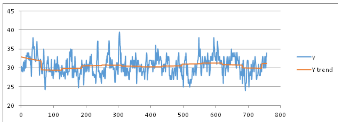
Figure 5. Trend of the max temperature in the months of July and August (from 1 July 2003 to 16 August 2015) obtained by using a best fit polynomial of nine degree.
