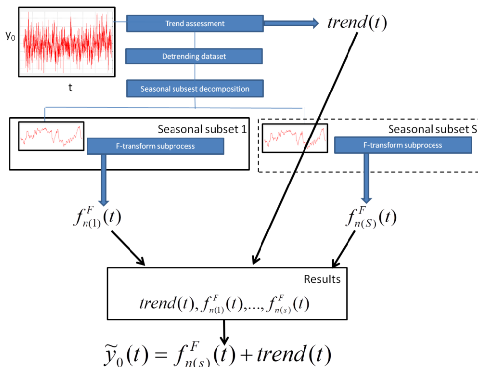
Figure 2. The TSSF method for forecasting analysis.
