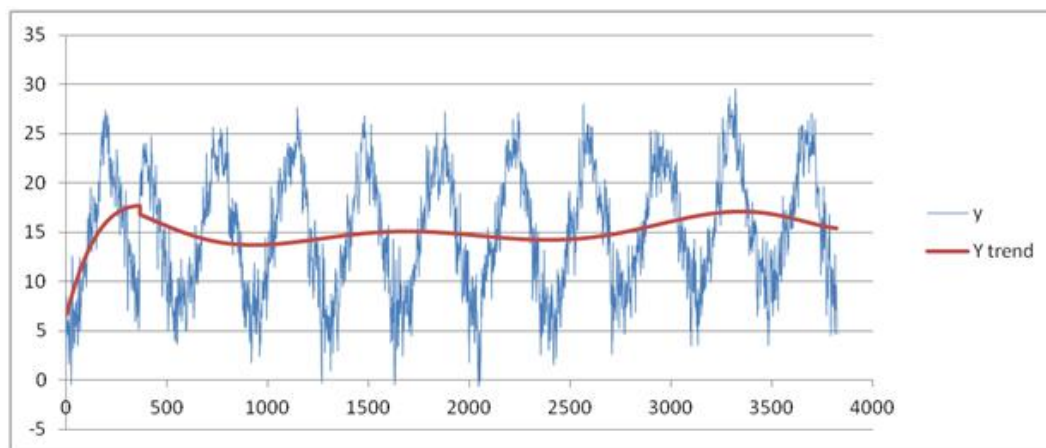
Figure 10. Trend of mean temperature under a best fit polynomial of nine degree Chiavari-Caperana weather station dataset.
