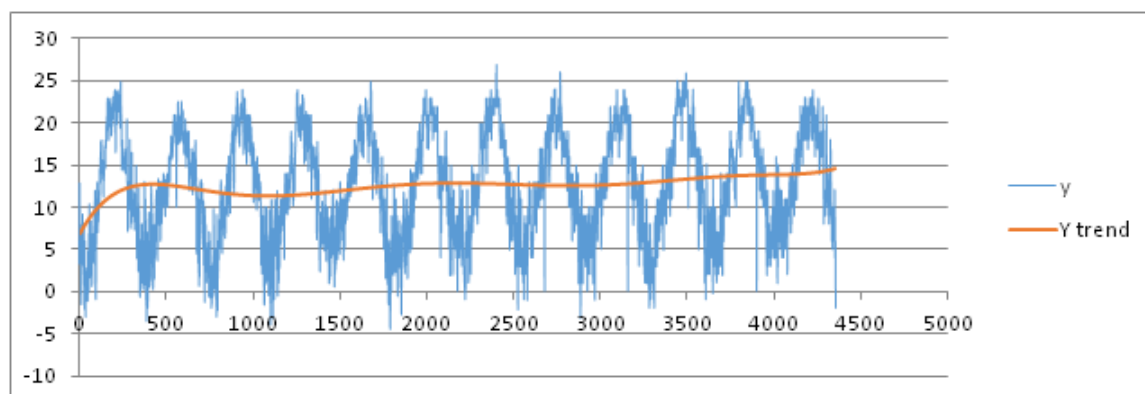
Figure 8. Trend of min temperature under a best fit polynomial of nine degree.
