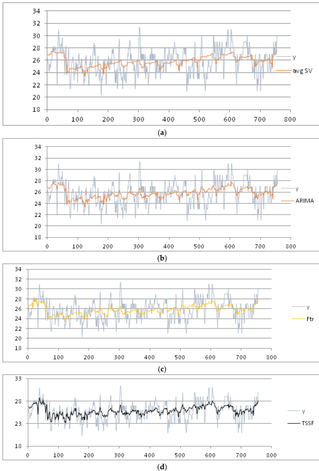
Figure 6. (a) Results obtained for the mean temperature by using the avgSV method; (b) results obtained for the mean temperature by using the ARIMA method; (c) results obtained for the mean temperature by using the F-transforms method; and (d) results obtained for the mean temperature by using the TSSF method.
