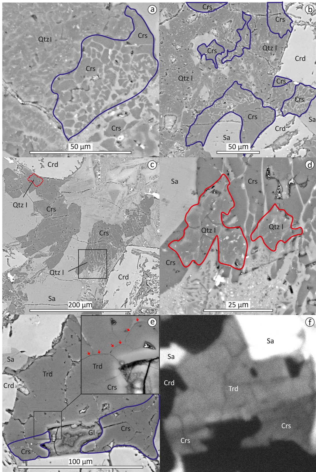
Figure 2. BSE (a–e) and CL (f) images of cristobalite occurrences with quartz (Qtz I) (c–f) and tridymite (e,f). Qtz—quartz, Trd—tridymite, Sa—sanidine, Crd—cordierite, Gl—glass. The blue outline shows the boundaries of cristobalite (a,b,e), the red outline shows the boundaries of quartz (c,d). The black square in (e) shows the corresponding enlarged fragment. Red arrows point to boundary of ballen tridymite.
