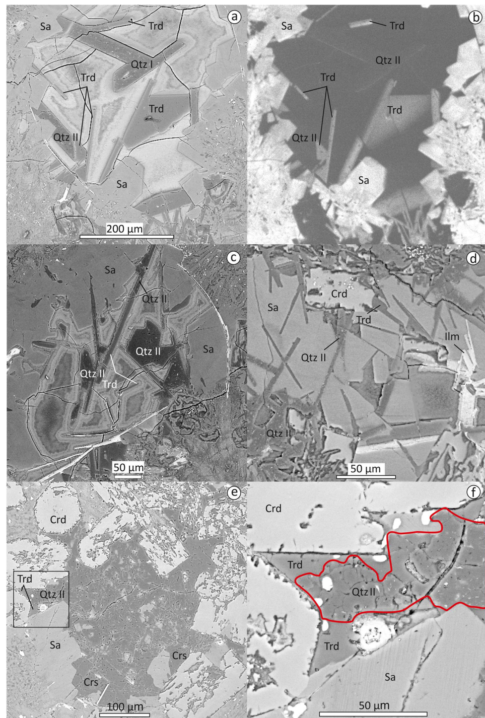
Figure 3. BSE images (a,c–f) and CL images (b) of tridymite (Trd) with quartz (Qtz II). Black square in (e) shows the contour of the enlarged fragment (f). Qtz—quartz, Trd—tridymite, Sa—sanidine, Crd—cordierite, Ilm—ilmenite.
