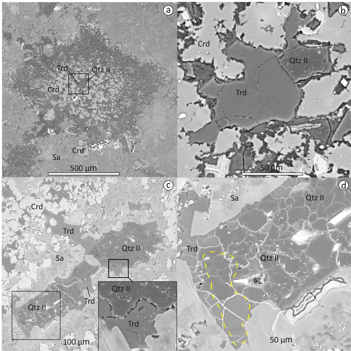
Figure 4. BSE images of ballen tridymite (Trd) with ballen quartz (Qtz II). The black square (a,c) shows contours of enlarged fragments (b,d), respectively. Yellow dotted line (d) shows the EBSD mapping region (Figure 5). Qtz—quartz, Trd—tridymite, Sa—sanidine, Crd—cordierite.
