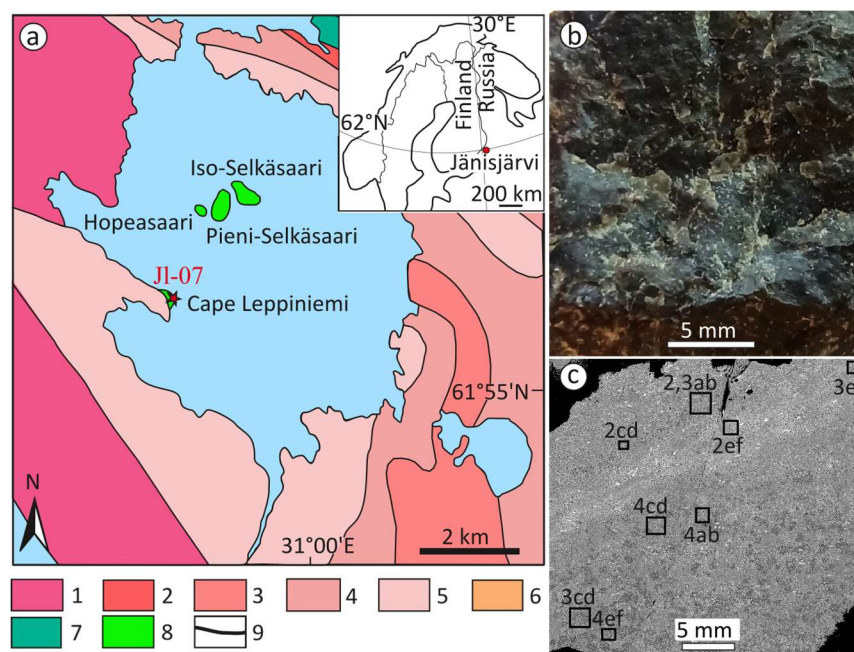
Figure 1. Schematic geological map with the geographical location in inset map of the Jänisjärvi structure (a), sample JI-07 (b) and a BSE image of polished thin section of the sample (c). Crater position is marked with red circle; sampling location of JI-07 is marked with red asterisks; 1—Pälkjärvi formation; 2–5—Naatselkä formation (2—undivided, 3—lower, 4—middle and 5—upper); 6—Early/Middle Proterozoic rocks; 7—gabbrodiabase; 8—impactites; 9—faults. Modified after [31]. Annotations in (c) describe the corresponding figures.
