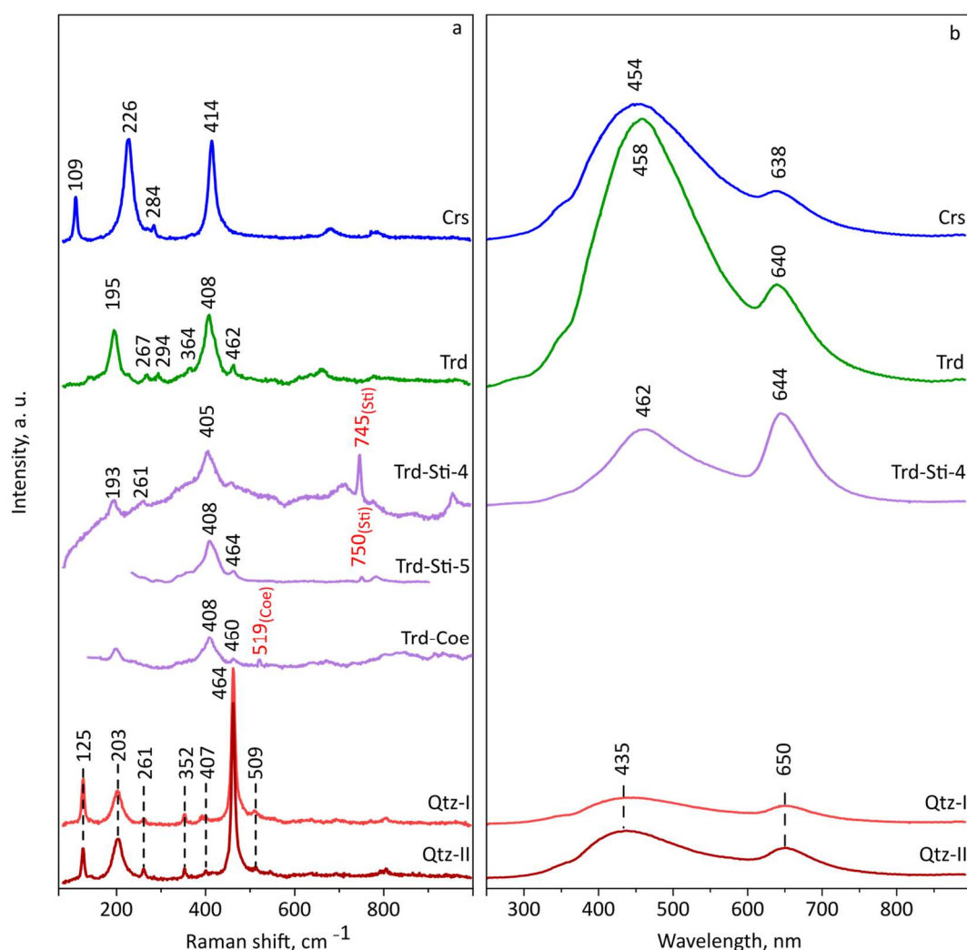
Figure 6. Raman (a) and CL (b) spectra of cristobalite (Crs), tridymite (Trd), tridymite with traces of stishovite (Trd-Sti) and coesite (Trd-Coe) and \alpha -quartz (Qtz I, Qtz II). Spectra of stishovite traces taken from point (4) and from region (5) shown in Figure 7.
