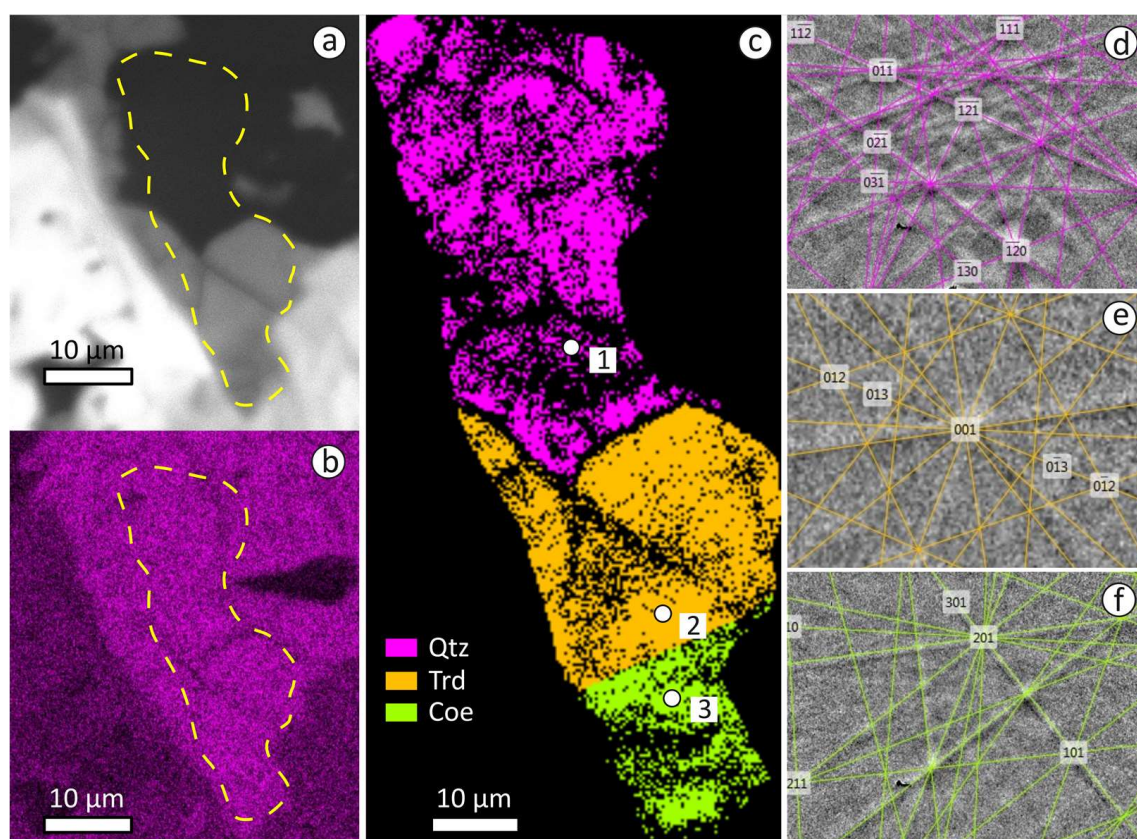
Figure 5. CL image (a), EDS map of Si distribution (b), phase EBSD map (c) of quartz, tridymite and trace coesite; (d–f)—indexed Kikuchi patterns of quartz (1), tridymite (2) and coesite (3) marked in (c). Yellow dotted line shows the EBSD mapping region.
