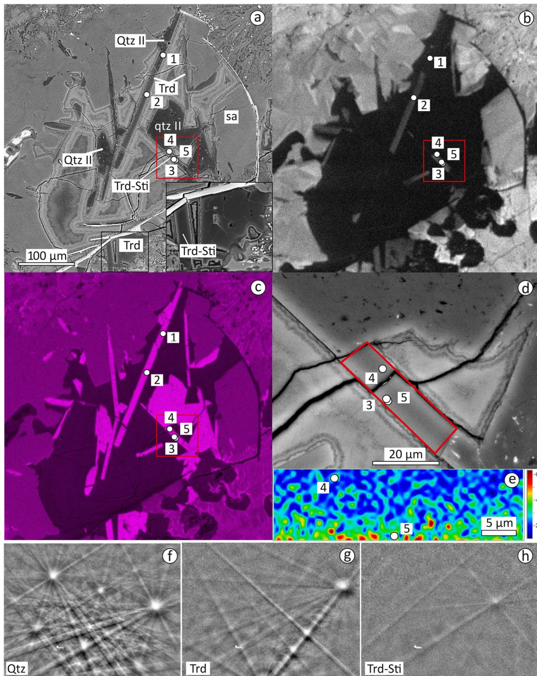
Figure 7. BSE (a) and CL (b) images and Si distribution EDS map (c) of tridymite, quartz and trace stishovite. Red square in (a–c) shows the contour of the enlarged fragment (d); the red outline in (d) outlines the area where Raman mapping was performed (e); the color-coded map (e) shows the intensity of the stishovite Raman band ( 746\text{--}751\text{ cm}^{-1} ) relative to the noise, with annotations for the point (4) and area (5) corresponding to the Raman spectra (Figure 6a). (f–h)—Kikuchi patterns corresponding to points 1 (quartz), 2 (tridymite) and 3 (tridymite with trace stishovite) on (a). Qtz—quartz, Trd—tridymite, Sa—sanidine, Sti—stishovite.
