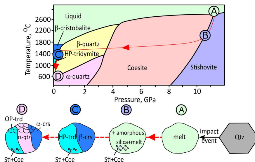
Figure 8. Schematic diagram of the P-T trajectory of silica from the Janisjärvi impact structure. The P-T-diagram is modified after [38].
