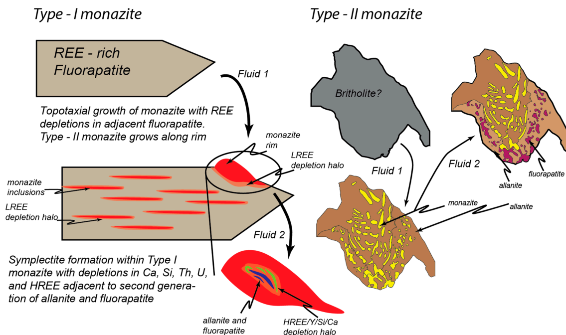
Figure 6. Schematic drawing proposing the reaction history and textural evolution of monazite-allanite-fluorapatite assemblages discussed in this study.
