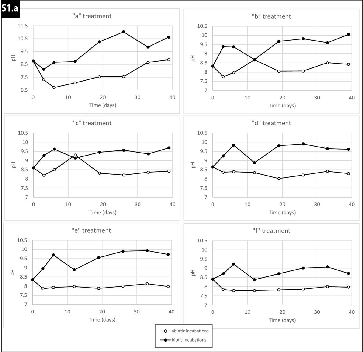
Supplementary Figure S1: Time serial development in all six experimental treatments: (S1.a) the pH, (S1.b) the \text{Ca}^{2+} concentration, (S1.c) the \text{HCO}_3^- concentration and (S1.d) the saturation index (SI) of calcite. Open symbols show abiotic controls (blanks), closed symbols depict biological treatments
