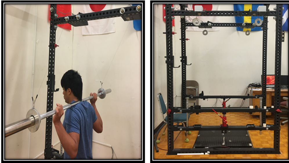
Figure S1. Set-up configuration of linear position transducers for data collection.
