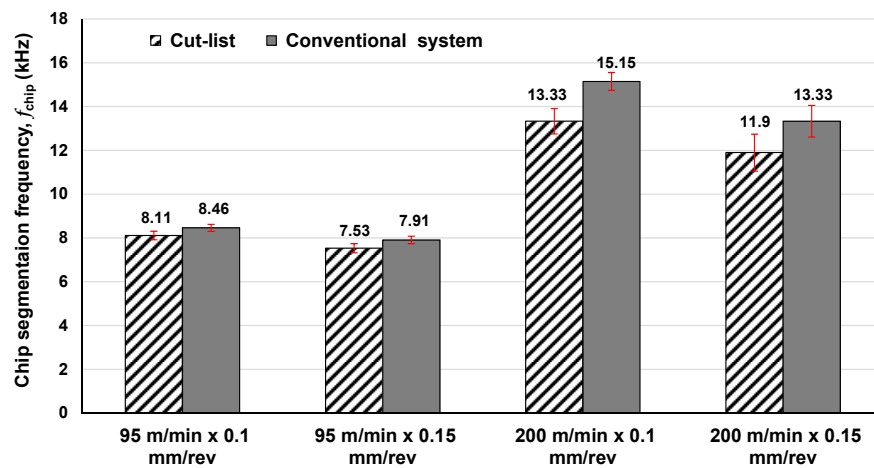
Figure 21. Frequency of segmentation at various cutting conditions for the two supply systems.
