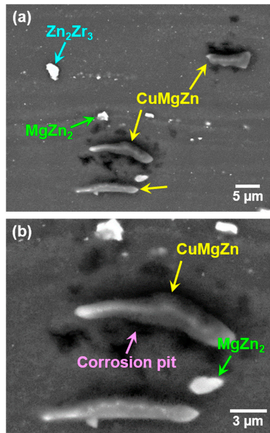
Figure 5. SEM micrographs showing the corroded surface of the ZKC601 alloy after immersion for 1 h in 0.6 M NaCl solution at 25 °C at relatively (a) low and (b) high magnifications.
