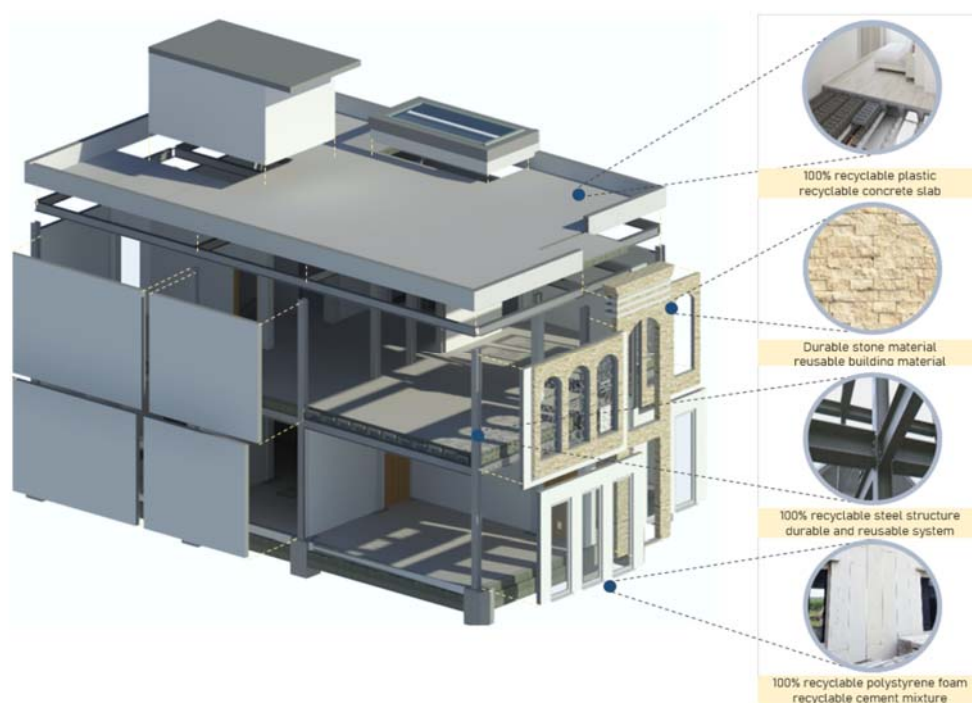
Figure 12. 7D BIM Application: Deconstruction Theme.
