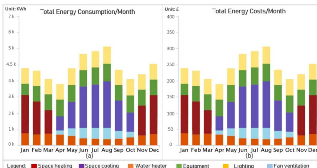
Figure 11. Standard Housing Unit: (a) Energy Consumption Analysis per Month, (b) Energy Costs per Month.
