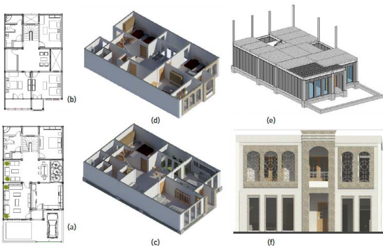
Figure 2. Prefabrication prototype; (a) Ground floor plan, (b) First floor plan, (c) Ground floor model, (d) First floor Model, (e) Unit structure (prefabrication elements), (f) House unit model.
