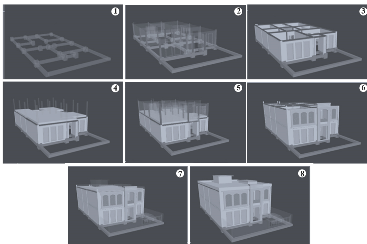
Figure 6. Simulating construction timeline with BIM from foundation to completion.
