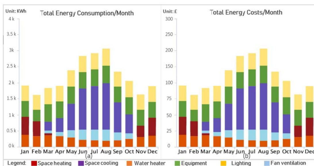
Figure 10. Prefabrication Unit: (a) Energy Consumption Analysis per Month, (b) Energy Costs per Month.
