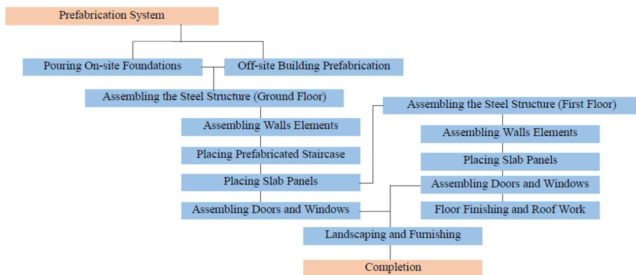
Figure 4. Work breakdown structure of the proposed housing paradigm.
