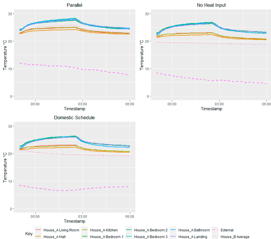
Figure 10. Example QUB temperature evolution for each heating pattern (Tests 1, 4 and 8).
