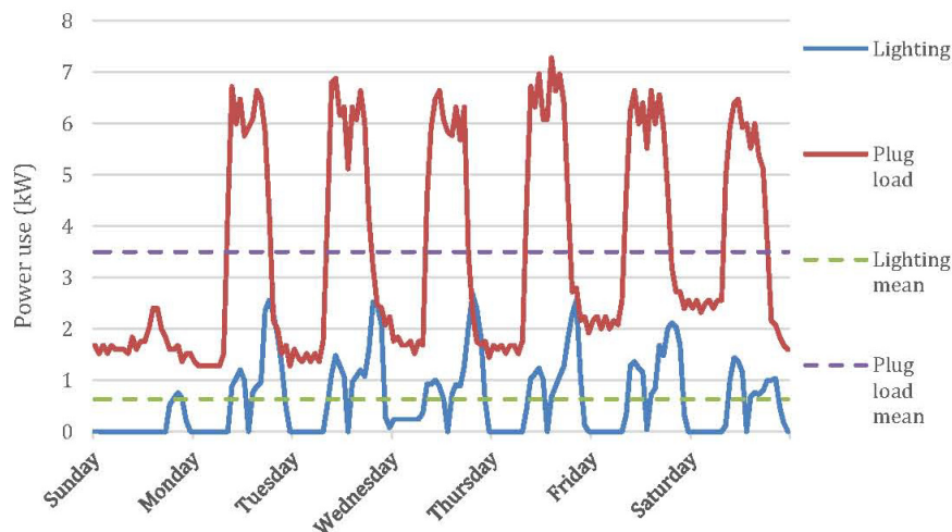
Figure 8. Power use for Plug Loads (red) and Lights (blue) for one week (1–7 August 2011) from the 8th floor offices of the IBR Building.
