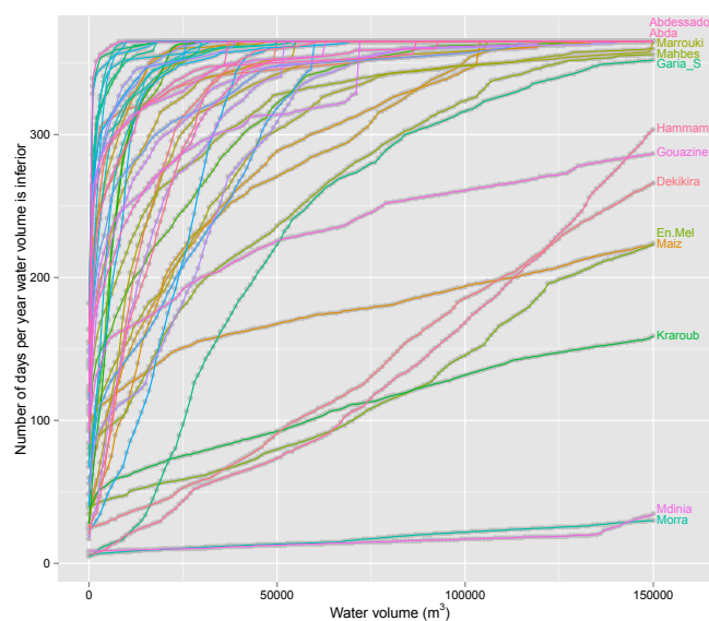
Figure 17. Number of days for each lake that water volumes fell below a designated volume (up to 150,000 m³).
