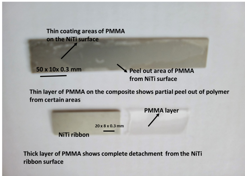
Fig. SM1 Images of the polymer PMMA on Ni-Ti surface without laser lines showing a detachment from the surface.
