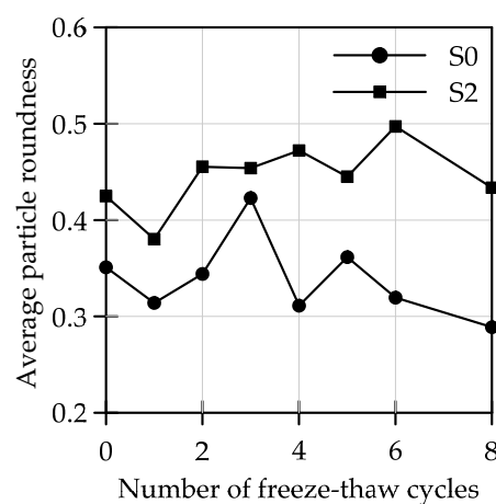
Figure 7. The curve of R and F-T cycles.
