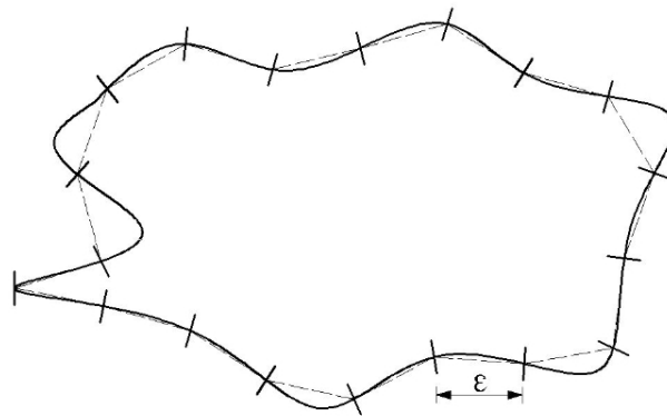
Figure 8. Schematic diagram of the D_{pr} algorithm.
