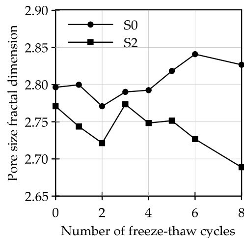
Figure 14. The curve of D_{hs} and F-T cycles.
