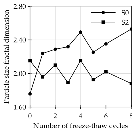
Figure 5. The curve of D_{ps} and F-T cycles.
