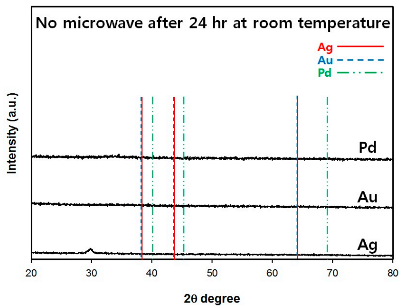
Figure S1. XRD patterns of synthesized Ag, Au, and Pd samples at room temperature without microwave irradiation. It shows no metal particles formation without microwave irradiation.
