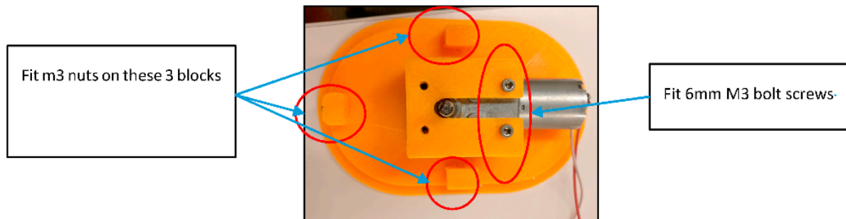
Figure 9. Base assembly.
