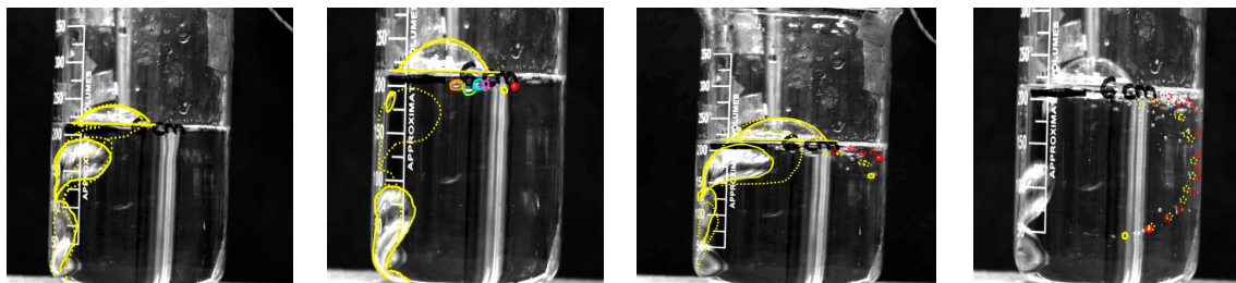
Figure 6. Pictures of the initial stages of bubbling when the small bubbles created at the free surface are captured by the liquid and entrained in its movement. Bubbles dragged by the liquid flow are highlighted by yellow and red circles.
