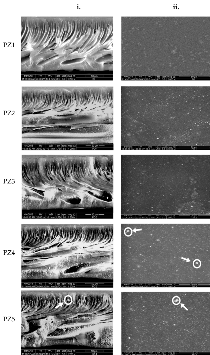
Figure S1. SEM micrographs of PZ1, PZ2, PZ3, PZ4 and PZ5 membrane (i) cross-section at 1200× magnification and (ii) Top surface at 2000× magnification.
