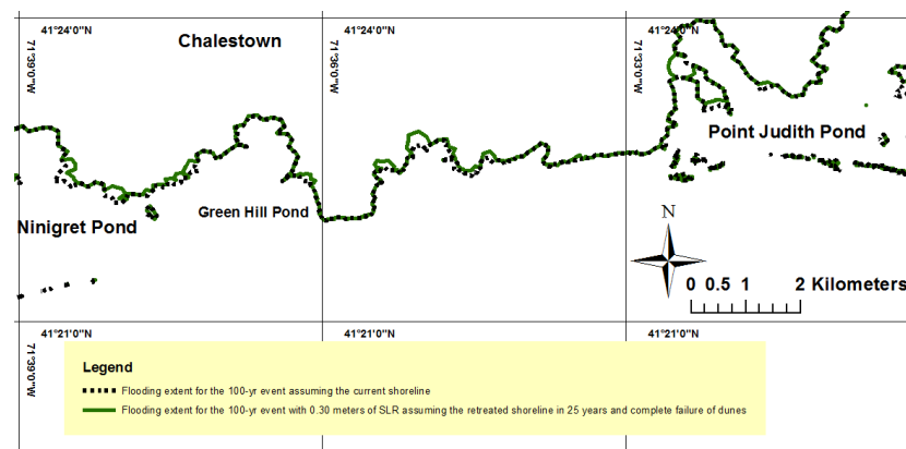
Figure 17. Comparison of flooding extend of the 100-year storm event, assuming 30 cm SLR, and coastal erosion.
