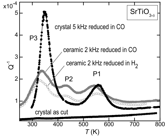
Figure 2. Elastic energy loss, Q^{-1} , of ceramic and single crystal \text{SrTiO}_{3-\delta} in the virgin state and after reduction in CO or \text{H}_2 atmosphere.
