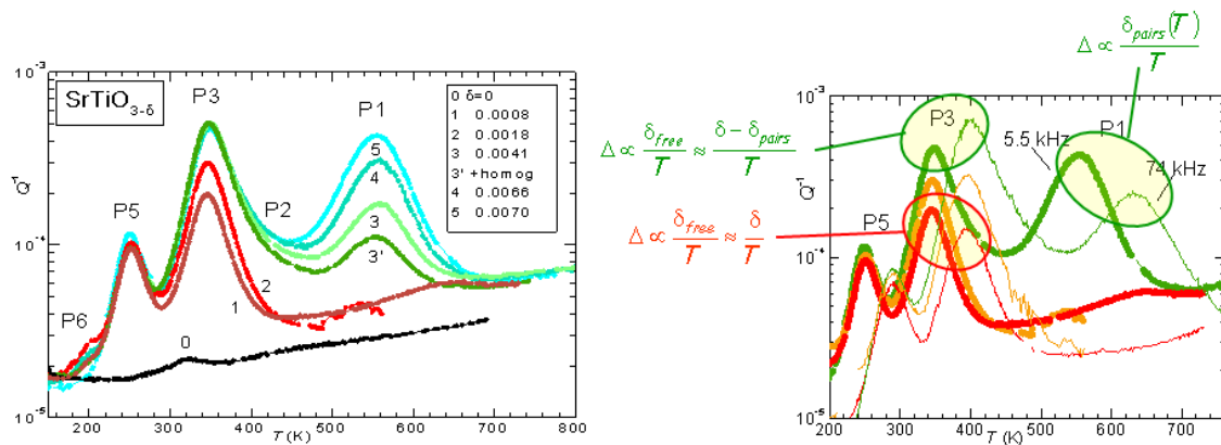
Figure 3. Elastic energy loss, Q^{-1} , of single crystal \text{SrTiO}_{3-\delta} at various levels of O deficiency measured at 5.5 kHz. Right side: Q^{-1}(T) curves measured at 5.5 and 74 kHz for \delta = 0.0008, 0.0018 and 0.0070 . Adapted with permission from Ref. [26], copyrighted by the American Physical Society.
