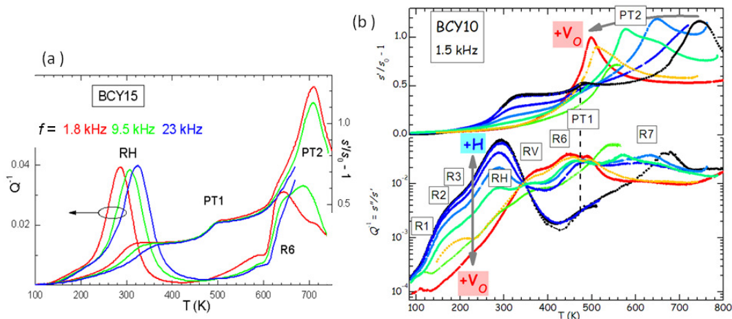
Figure 5. (a) Elastic energy loss and compliance s' normalized to its value s_0 at 0 K of hydrated BaCe_{1-x}Y_xO_3 with x = 0.15 , measured during the same run at three frequencies; (b) Elastic energy loss and normalized compliance of BaCe_{1-x}Y_xO_3 with x = 0.10 at different levels of hydration and outgassing. The thermally activated relaxation processes are labelled as R_x , while the phase transitions with PT_x . The arrows indicate the sequence according to increasing hydration (+H) or outgassing (+ V_O ).
