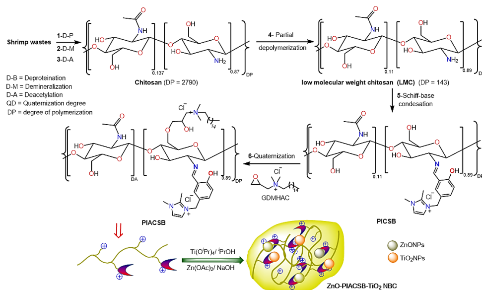
Figure 1. Step-by-step synthesis of PIACSB and ZnO-PIACSB-TiO 2 NBC.
