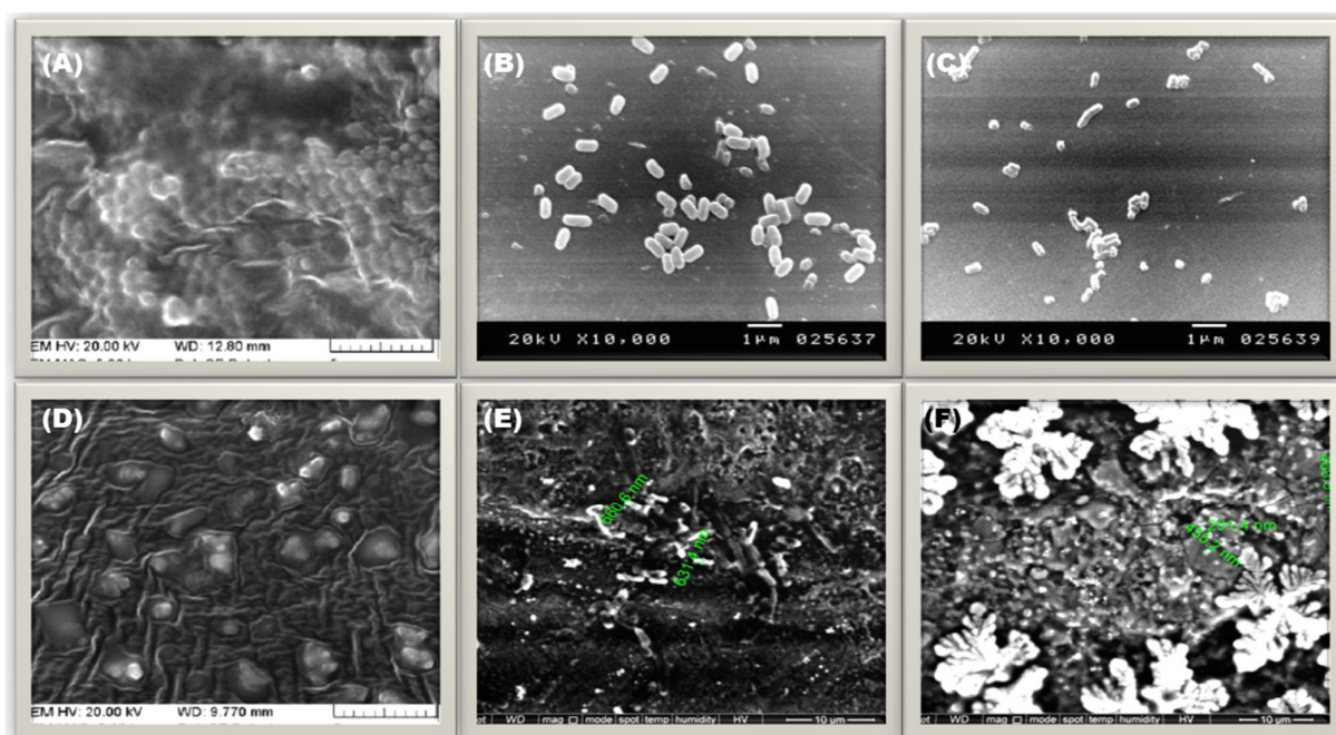
Figure 6. (A–C) SEM micrographs of the untreated (control) bacterial cell cultures (A) S. aureus , (B) E. coli , and (C) P. aeruginosa . (D–F) SEM micrographs of the NBC-treated (control) bacterial cell cultures (D) S. aureus , (E) E. coli , and (F) P. aeruginosa . The scale for pictures (A–D) is 1 µm, while for pictures (E,F), it is 10 µm.
