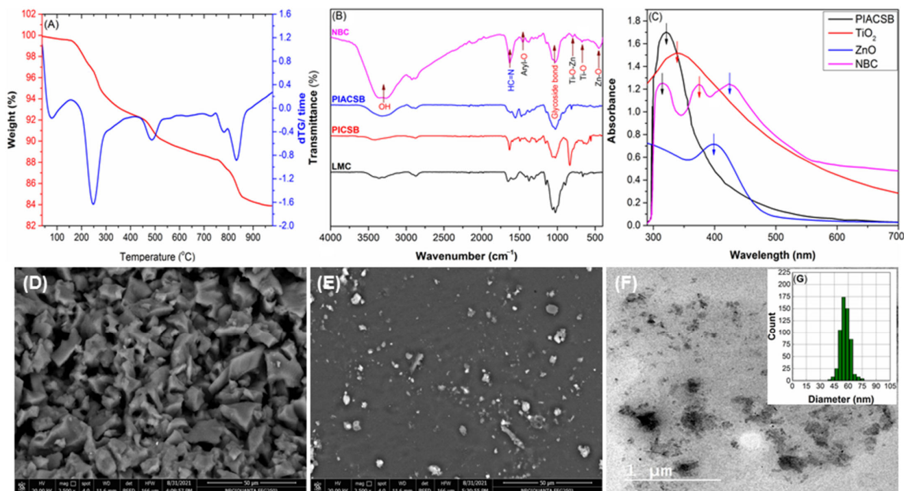
Figure 2. (A) Thermogravimetric analysis (TGA) and differential thermal analysis (DTA) curves of the ZnO-PIACSB-TiO 2 NBC. (B) FTIR spectra of newly produced materials displaying the key, recognizable absorption bands. (C) UV-Vis spectra of the obtained materials displaying the key, recognizable electronic transition peaks. (F) SEM microimages of (D) PIACSB and (E) ZnO-PIACSB-TiO 2 NBC. (F) TEM nanoimage of the ZnO-PIACSB-TiO 2 NBC. (G) PSD histograms of the ZnO-PIACSB-TiO 2 NBC. Arrows in (C) refer to the characteristic functional groups of each material.
