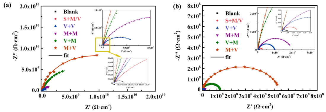
Figure S1. Nyquist plots of AA2024 coated with different coatings immersed in 3.5 wt.% NaCl solution for (a) 2 and (b) 10 days.
